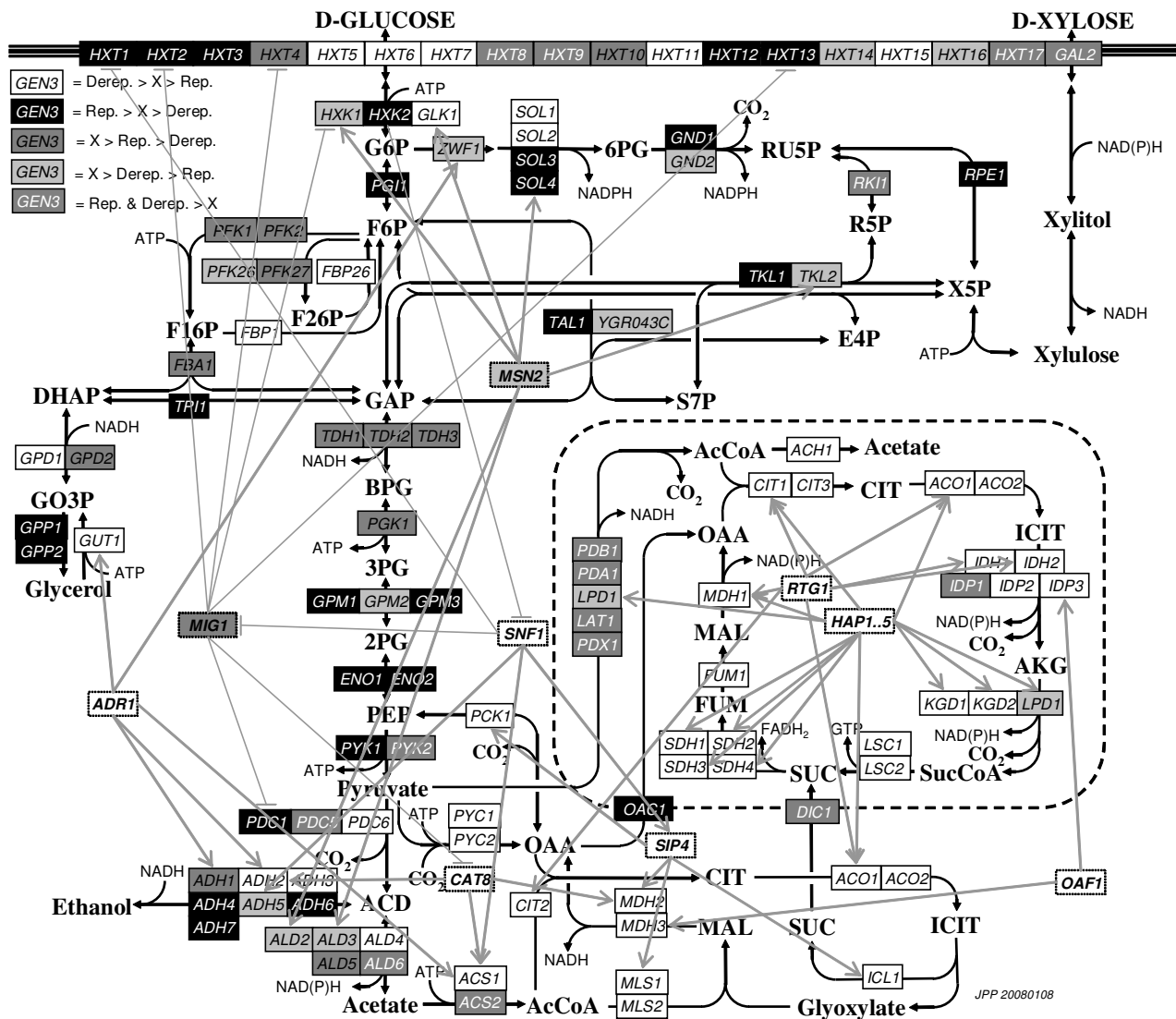
Figure 3 Expression profiles of genes involved in the main metabolic networks of S. cerevisiae . Transcription factors are presented with boldfacing and connected to the respective target genes with gray lines. The connections shown between transcription factors and their target genes are based on compilations in Yeast Proteome Database [70][80] and on the transcription factor binding network by Young and co-workers [82]. Expression of the genes presented in white boxes with black text was highest in the glucose derepressed cells (Derép.) and lowest in the glucose repressed cells (Rep.). Expression of the genes presented in black boxes with white text was highest in the glucose repressed cells and lowest in the glucose derepressed cells. Expression of the genes presented in dark gray boxes with black text was highest in the xylose-grown cells and lowest in the glucose derepressed cells. Expression of the genes presented in light gray boxes with black text was highest in the xylose-grown cells and lowest in the glucose repressed cells. Expression of the genes presented in gray boxes with white text was lowest in the xylose-grown cells. In addition to the genes shown in the figure, 89% of the genes (31 out of 35) annotated to GO category "Oxidative phosphorylation" and its daughter categories [33] had highest expression in the glucose derepressed cells, lowest expression in the glucose repressed cells and intermediate expression in the cells grown on xylose (data not shown).
