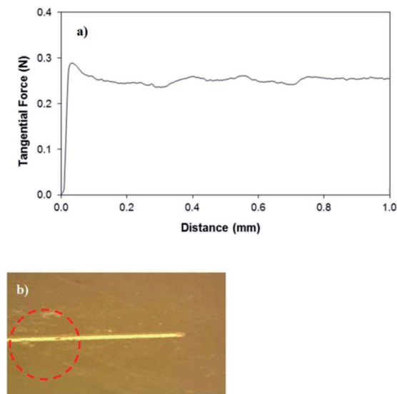
Fig. 5 Tangential force measured by a micro-tribometer for silica particle removal from the glass surface and an optical image of the scratch mark: (a) tangential force, and (b) optical image of the scratch mark. Residues of functionalized silica particles on the indentation path.
