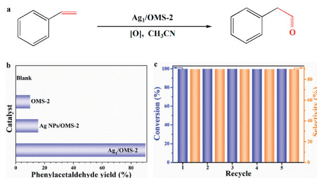
Fig. 3 (a) Scheme of Wacker oxidation of styrene. (b) Phenylacetaldehyde yield of different catalysts. (c) Recycling test of \text{Ag}_1/\text{OMS-2} for the catalytic Wacker oxidation of styrene.
