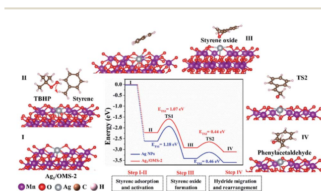
Fig. 5 DFT calculation proposed a reaction pathway for the Wacker oxidation of styrene to phenylacetaldehyde on Ag 1 /OMS-2, and the calculated energy profiles for Ag 1 /OMS-2 (red line) and Ag NPs (blue line).
