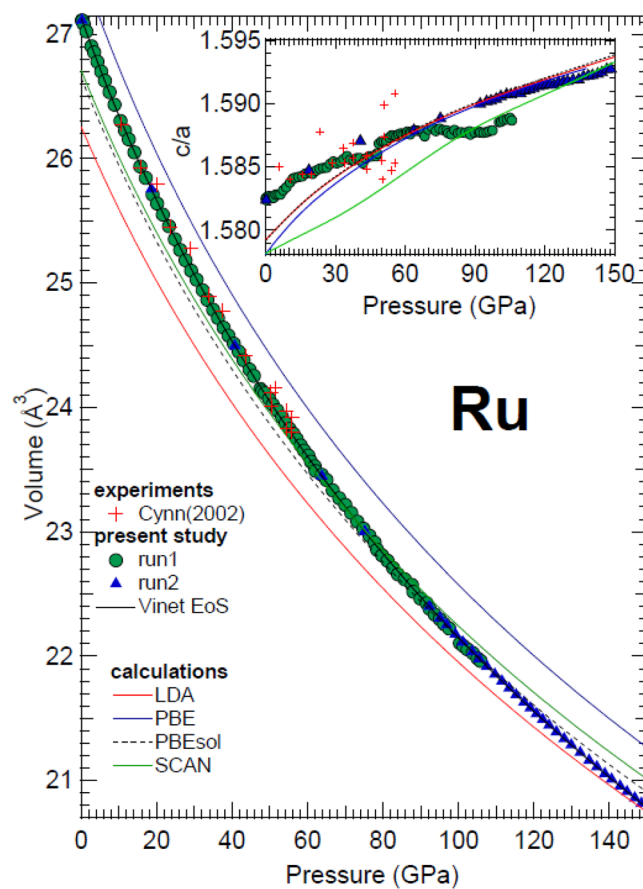
Figure 2. Measured and calculated volume of ruthenium as a function of pressure compared with literature data. Inset: evolution of the c/a ratio. Same symbols are used in both the main figure and the inset. In both figures the error bars are smaller than the used symbols.
