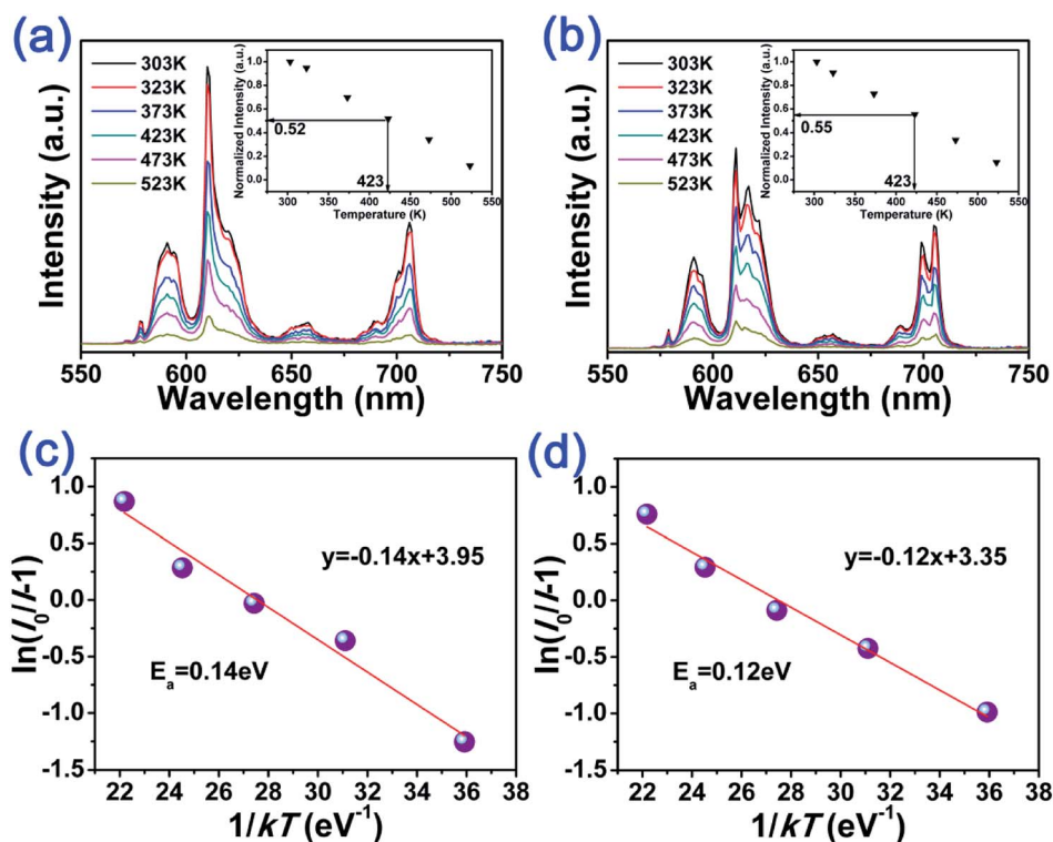
Fig. 3 Temperature-dependent PL spectra of (a) BEB:0.3Lu 3+ and (b) BEB phosphors excited at 395 nm (The insets show normalized PL intensity as a function of temperature.). The plots of \ln(I_0/I - 1) versus 1/kT and the calculated activation energy ( E_a ) for (c) BEB:0.3Lu 3+ and (d) BEB phosphors.
