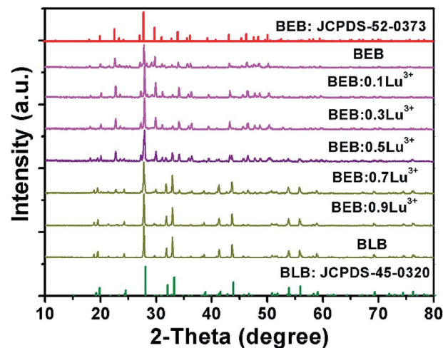
Fig. 1 XRD patterns of BEB:xLu 3+ ( x = 0, 0.1, 0.3, 0.5, 0.7, 0.9, \text{ and } 1.0 ) phosphors. The standard data of BLB (JCPDS-45-0320) and BEB (JCPDS-52-0373) were shown.
