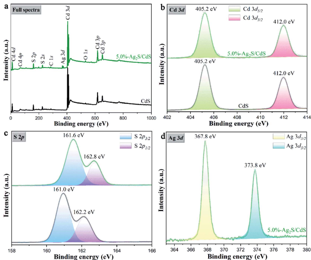
Fig. 7 (a) Full XPS survey spectra; and high-resolution XPS spectra of (b) Cd 3d, (c) S 2p and (d) Ag 3d of the CdS and 5.0%- \text{Ag}_2\text{S}/\text{CdS} nanocomposite.
