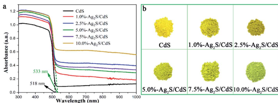
Fig. 6 (a) UV-vis DRS and (b) corresponding images of CdS and \text{Ag}_2\text{S}/\text{CdS} nanocomposites.
