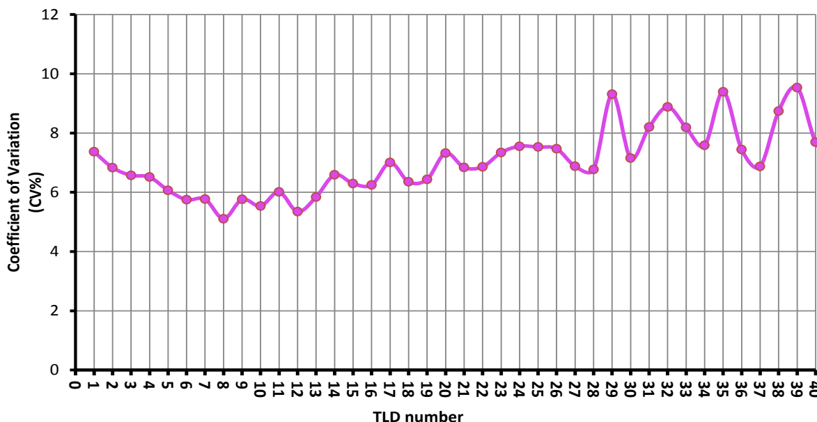
Figure 1: The coefficient of variation (CV%) for the response of each TLD
