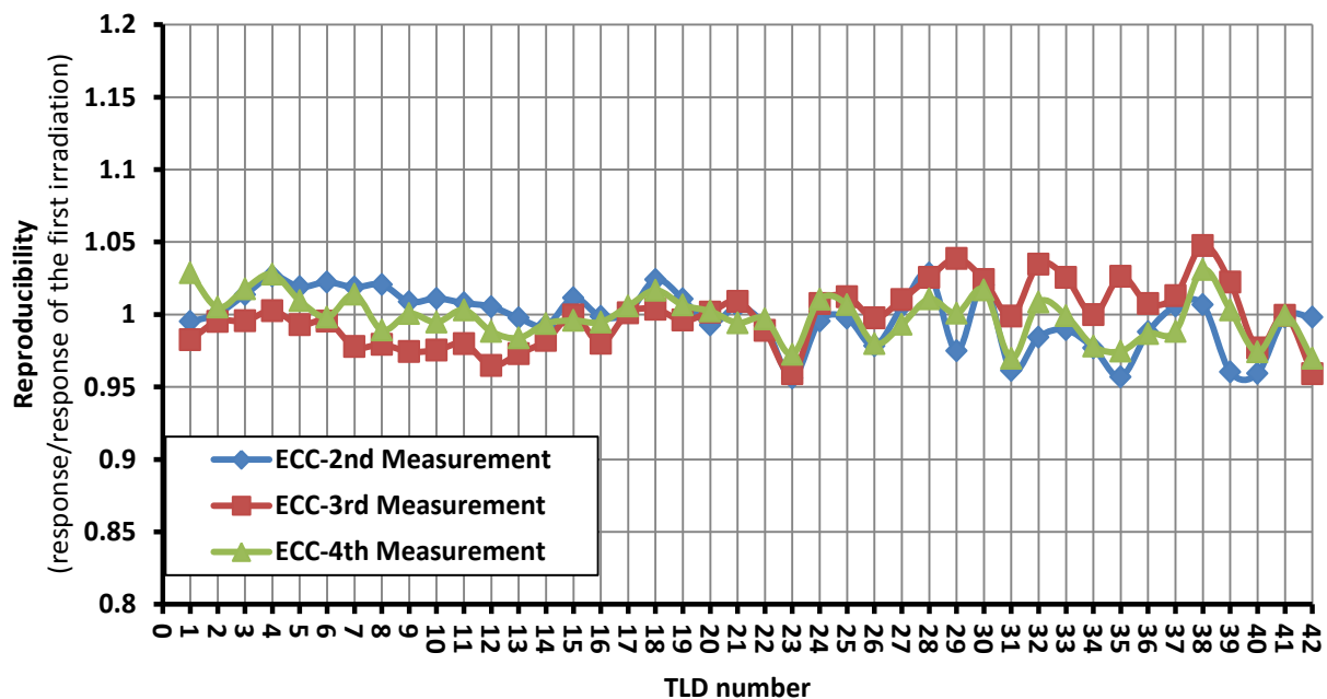
Figure 2: Reproducibility of the ECC
