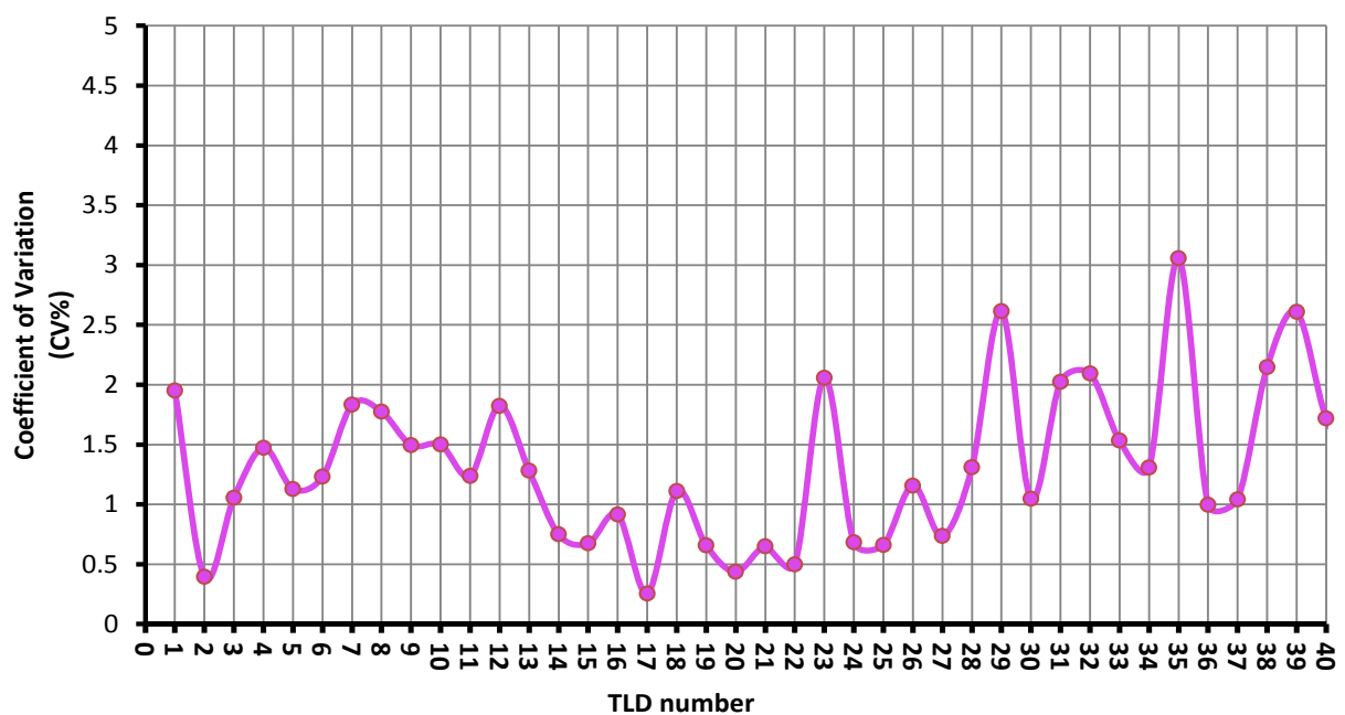
Figure 3: Coefficient of variation (CV%) for the ECC of each TLD
