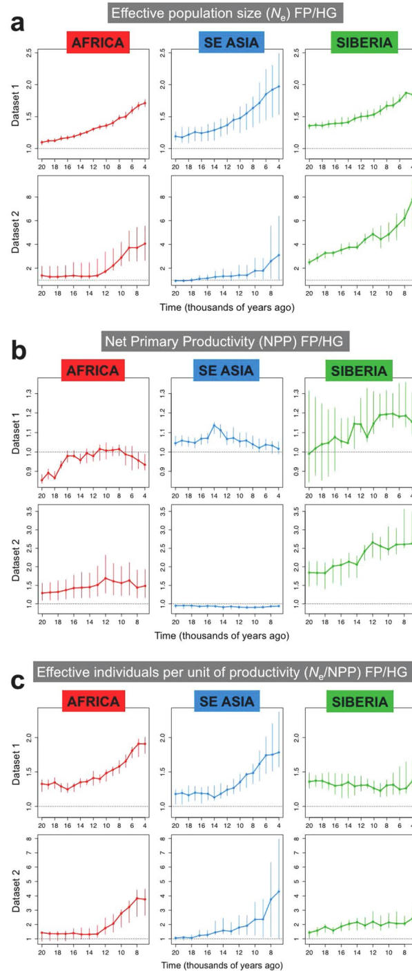
Figure 2. Median of the ratio of food producers over hunter-gatherers for N_e (a), NPP (b) and N_e/NPP (c) in the three regions considered: sub-Saharan Africa, south-eastern Asia and Oceania, and Siberia. The plots show the temporal range between 4,000 and 20,000 years ago for dataset 1 and between 7,000 and 20,000 years ago for dataset 2. The error bars represent the 95% distribution of the jackknife leave-one-out validation.
