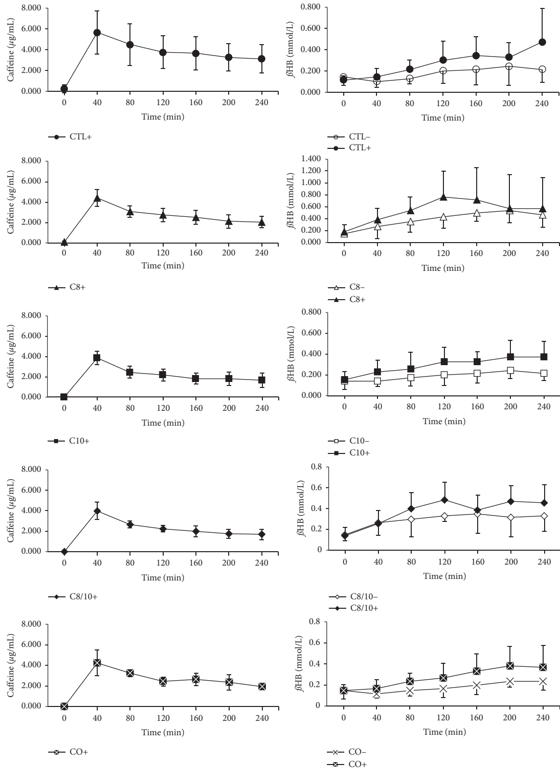
FIGURE 3: Overview of the curves (mean and standard deviation) of caffeine in saliva ( \mu\text{g/mL} ) from caffeinated interventions (CTL+, C8+, C10+, C8/10+, and CO+) and of \beta\text{HB} ( \text{mmol/L} ) in capillary blood during all interventions over 240 min ( t_0-t_6 ). The interventions containing caffeine are in black.
