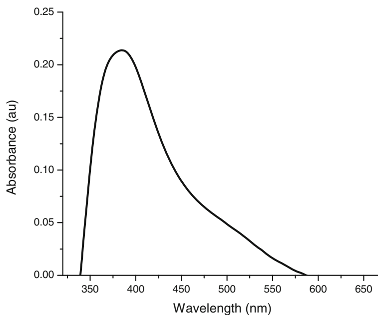
Fig. 2 UV-Vis spectroscopy of AgNPs reduced by chitosan
