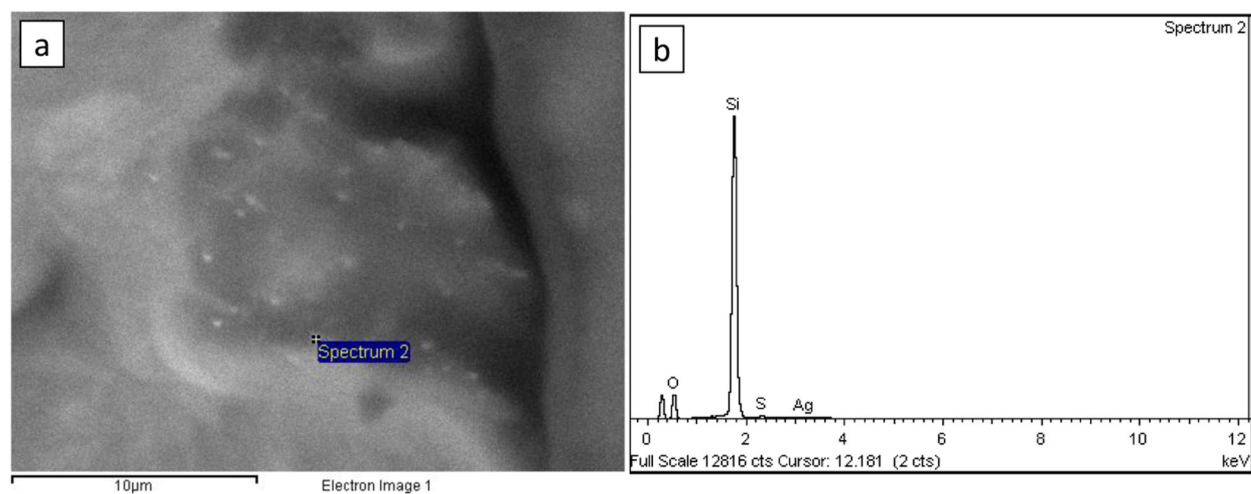
Fig. 4 SEM-EDX analyses of the composite. a distribution of AgNPs on the composite, b EDX spectrum of the composite with AgNPs
