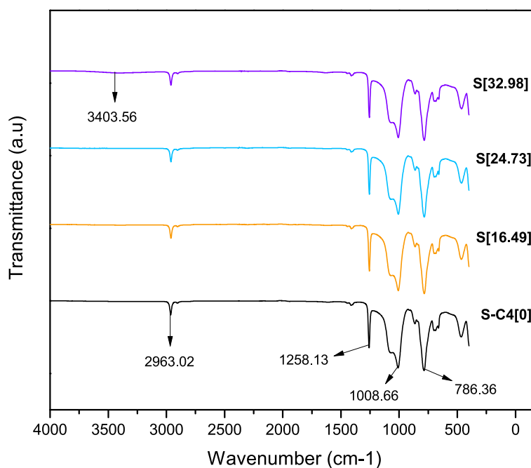
Fig. 5 FTIR spectrum of the composite with different concentrations of AgNPs
