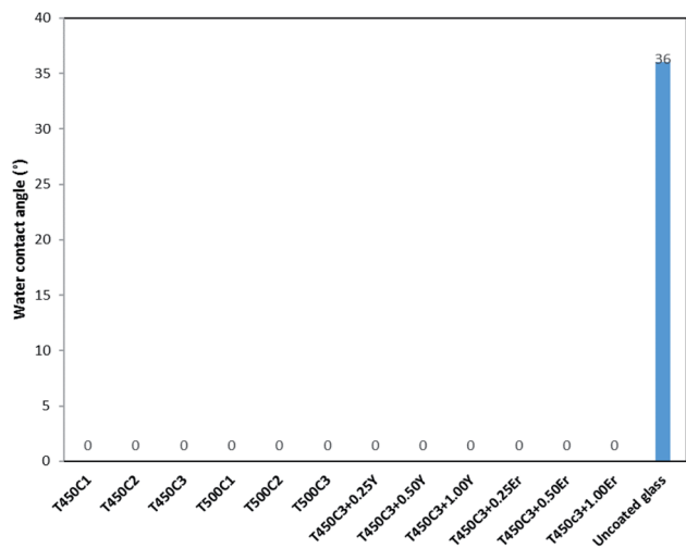
Fig. 4 Apparent water contact angles for the doped and undoped TiO 2 thin film glass after 24 h UVA irradiation.
