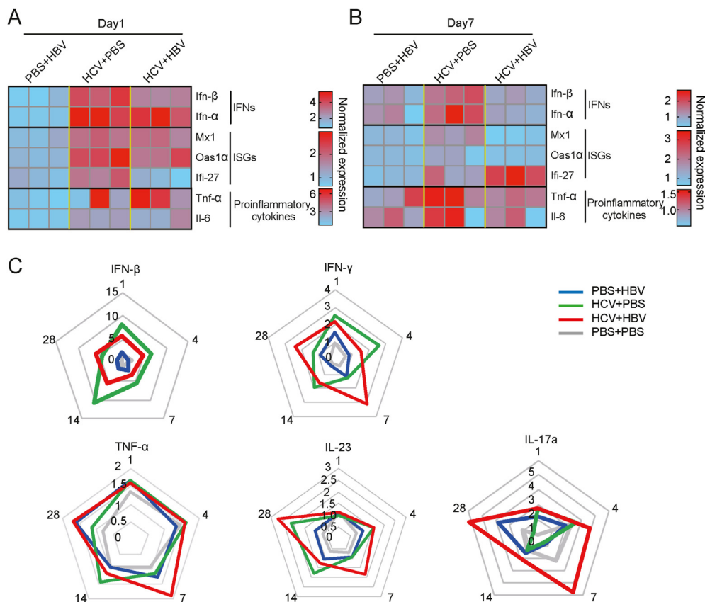
Fig. 5. Changes of innate immune response-related cytokines after coinfection. A–B Heatmaps show the RT-qPCR detection of mRNA levels of IFN- \alpha , IFN- \beta and ISGs Mx1 , Oas1a and Irfi-27 as well as inflammatory genes Tnf- \alpha , Il-6 in liver; three mice in each group. C Levels of serum cytokines IFN- \beta , IFN- \gamma , TNF- \alpha , IL-23, IL-17a at 1, 4, 7, 14, 28 days post infection were shown in radar plots as a fold change, which were calculated by dividing the baseline levels (day 0).
