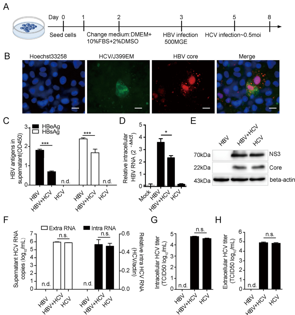
Fig. 1. HCV inhibits HBV replication while HBV does not affect HCV replication in coinfected Huh7-NTCP cells. A Schematic presentation of experiment design. Huh7-NTCP cells were treated DMEM medium containing 10% FBS and 2% DMSO before HBVcc infection which was followed by HCVcc infection to establish coinfection in vitro . B HBV core and HCV NS5A expressions. Scale bar = 100 \mu m. C Supernatant HBeAg and HBsAg. D Intracellular HBV RNA was tested by relative quantification using RT-qPCR. Gray dot dash indicates the baseline of the test. E HCV NS3 and core protein. F Extracellular and intracellular HCV RNA. G Intracellular and H extracellular HCV titers. The statistical significance is calculated using the two-tailed, unpaired t -test. *, P < 0.05 ; ***, P < 0.001 ; n.s., not significant ( P \geq 0.05 ); n. d. not detected.
