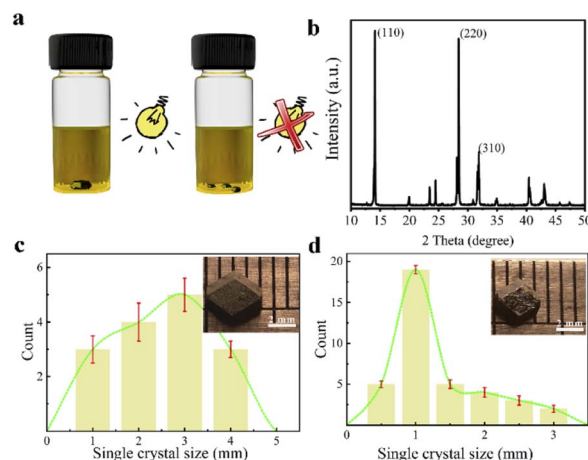
Fig. 1 (a) Growth processes of \text{MAPbI}_3 crystals under light and dark conditions, the light intensity of which is 64 \text{mW cm}^{-2} . (b) XRD curves for \text{MAPbI}_3 single crystal. And the statistical data of the size and number of \text{MAPbI}_3 single crystals in their precursor solutions under light (c) and dark (d) conditions, respectively. The insert images are the \text{MAPbI}_3 single crystal grown from its precursor solution after 36 h.
