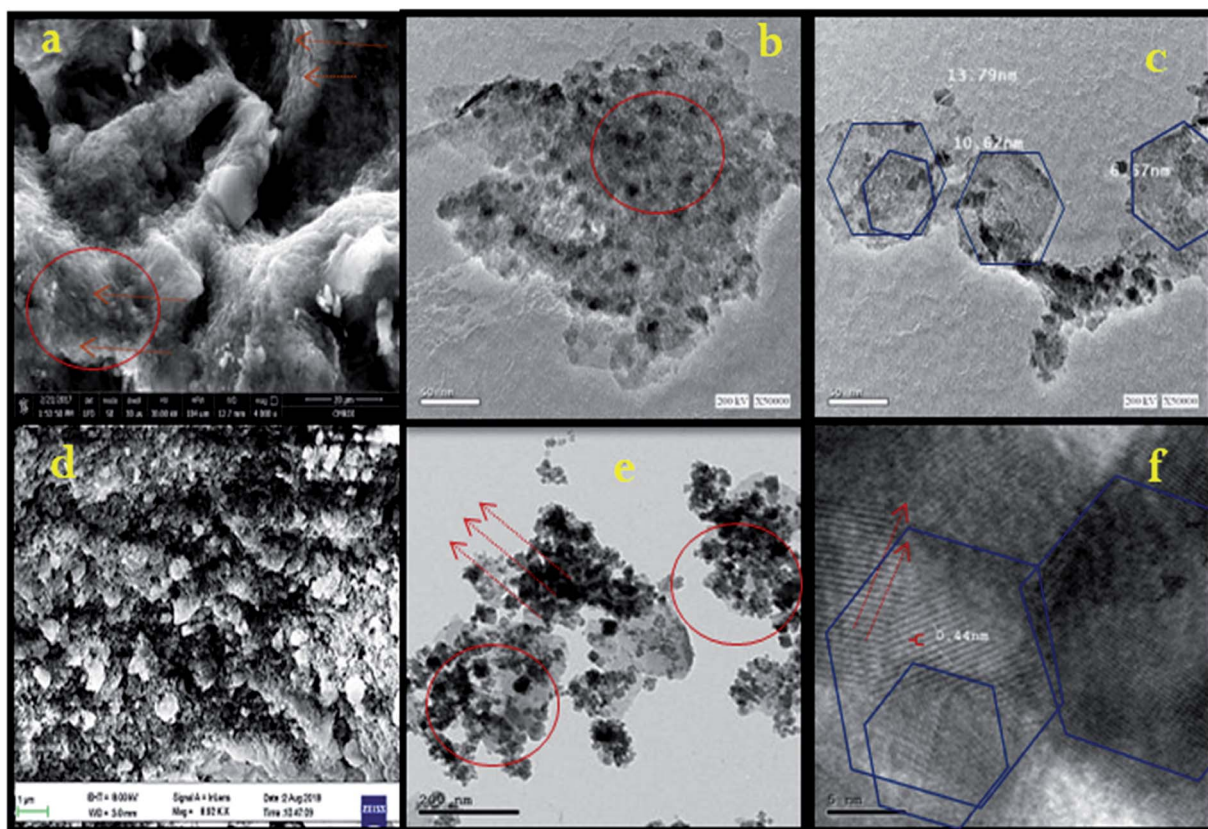
Fig. 3 (a) FESEM image of the Co-Fe LDH before irradiation, (b) and (c) HR-TEM images of Co-Fe LDH before irradiation, (d) FESEM image of Co-Fe LDH after irradiation and (e) and (f) HR-TEM images of Co-Fe LDH after irradiation.
