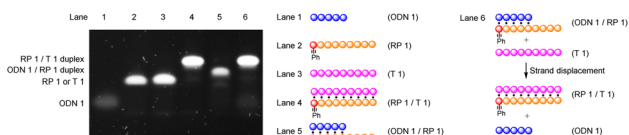
Fig. 3 Electrophoretic mobility shift assay to identify strand displacement reaction of ODN 1/RP 1 duplex by T 1 target. ODNs bearing alkyne tags (RP 1) were hybridized with their complementary strand (ODN 1). Then, T 1 was added to the sample and the resulting sample was loaded into 10% polyacrylamide gel. Lane 1, single stranded ODN 1; lane 2, single stranded RP 1; lane 3, single stranded T 1; lane 4, RP 1/T 1 duplex; lane 5 ODN 1/RP 1 partial duplex; lane 6, addition of T 1 to ODN 1/RP 1 partial duplex to form RP 1/T 1 duplex and single stranded ODN 1.
