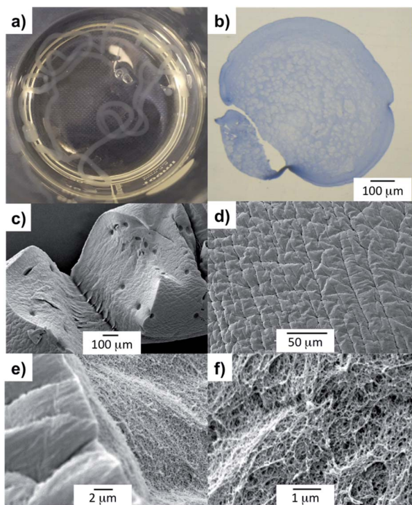
Fig. 2 DBS-CONH 2 H 2 /alginate gel tubes images. (a) Photographic image of the hybrid gel tube in CaCl 2 . (b) Optical microscopy image of the gel tube cross-section embedded in resin and stained with toluidine blue; scale bar: 100 μm. (c and d) SEM images of the gel tube surface; scale bars 100 μm (c) and 50 μm (d). (e and f) SEM images of the gel tube cross-section; scale bars 2 μm (e) and 1 μm (f).
