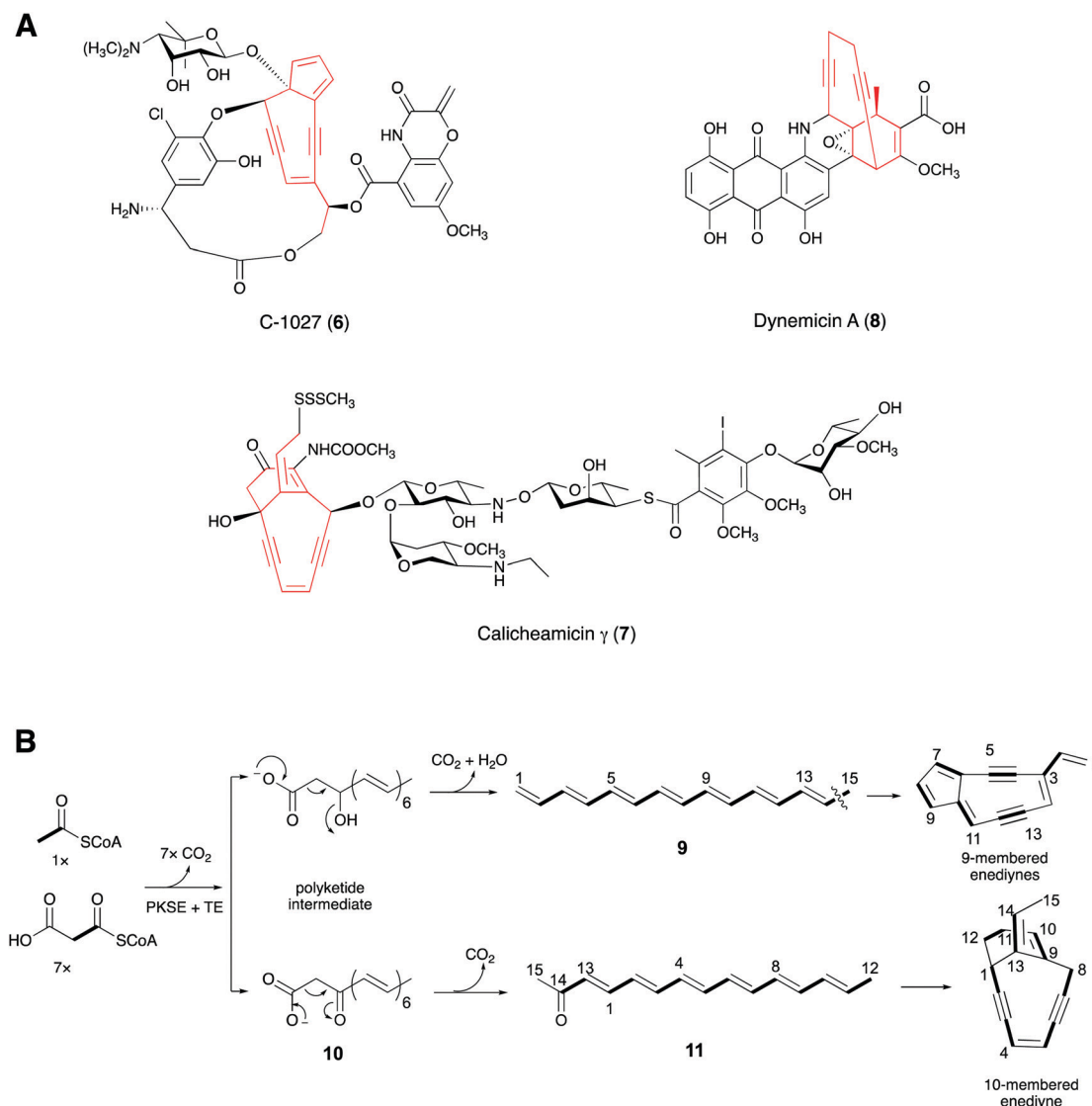
Fig. 5 (A) Structures of 6–8 . (B) Postulated biosynthetic routes to 9- and 10-membered enediyne.
