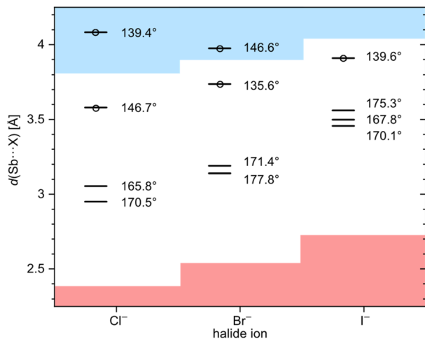
Fig. 4 Diagram of the four Sb...X distances of [2·Cl] - [Me 4 N] + , [2·Br] - [ n Bu 4 N] + and [2·I] - [ n Bu 4 N] + in the solid state. The red area marks an Sb...X distance below the sum of the covalence radii, 65 the blue area a distance above the sum of the van der Waals radii. 61,62 In addition to these distances, the corresponding angle of each X...Sb-C F motif is given. Sb...X distances, for which the corresponding Sb-C F bond is not elongated (compared to the longest Sb-C F distance in free host 2; 2.244(6) Å) are marked with a circle. The numerical values of this figure are provided in the ESI.†
