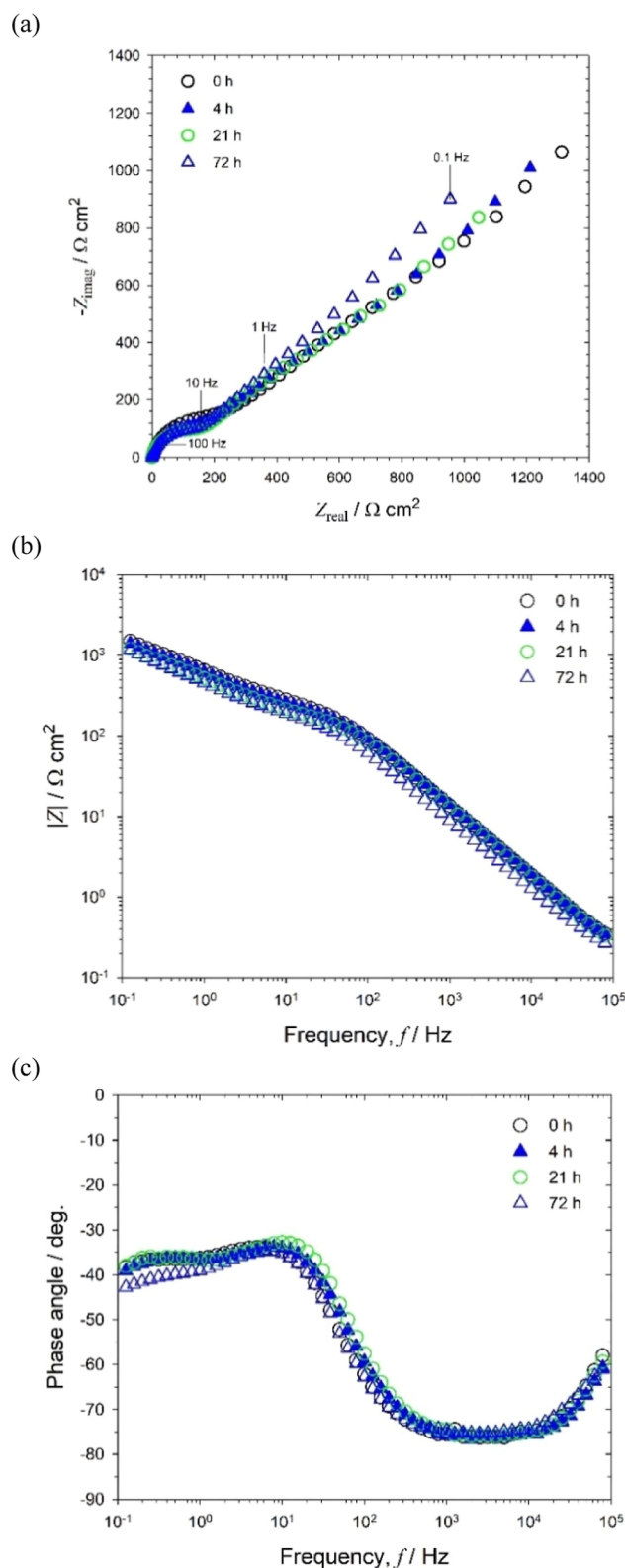
Figure 3. EIS for abiotic artificial seawater medium (#2): (a) Nyquist, (b) Bode |Z| , and (c) Bode phase angle at OCP: +0.085 , -0.070 , -0.250 , and -0.325 V after 0, 4, 21, and 72 h of immersion, respectively.
