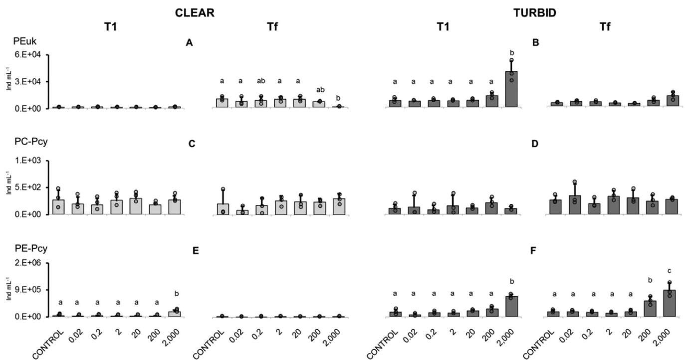
Fig. 6. A-F: Mean values (columns) and measurements of replicates (dots) of PPP population abundances ( \text{ind mL}^{-1} ) determined by flow cytometry at 15 min (T1) and 168 h (Tf). A. picoeukaryotes (PEuk); clear; B. picoeukaryotes (PEuk); turbid; C. phycocyanin-rich picocyanobacteria (PC-Pcy), clear; D. phycocyanin-rich picocyanobacteria (PC-Pcy), turbid; E. phycoerythrin-rich picocyanobacteria (PE-Pcy) clear; F. phycoerythrin-rich picocyanobacteria (PE-Pcy) turbid. Bars \pm 1 SD. Results were compared by a one-way ANOVA followed by Tukey's multiple comparisons test. Different letters mean significant differences ( p < 0.05 ).
