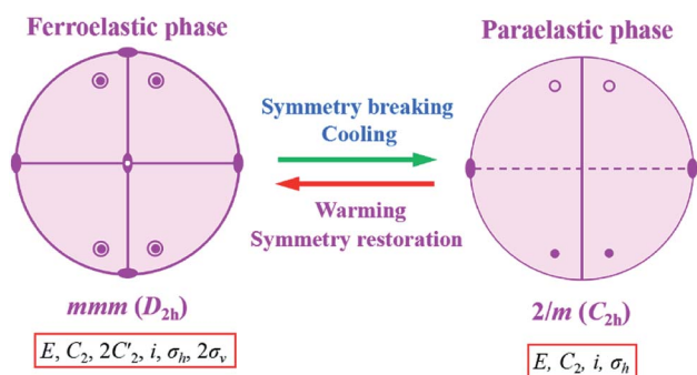
Fig. 7 Symmetric breaking diagram of complexes 1 and 2 .
