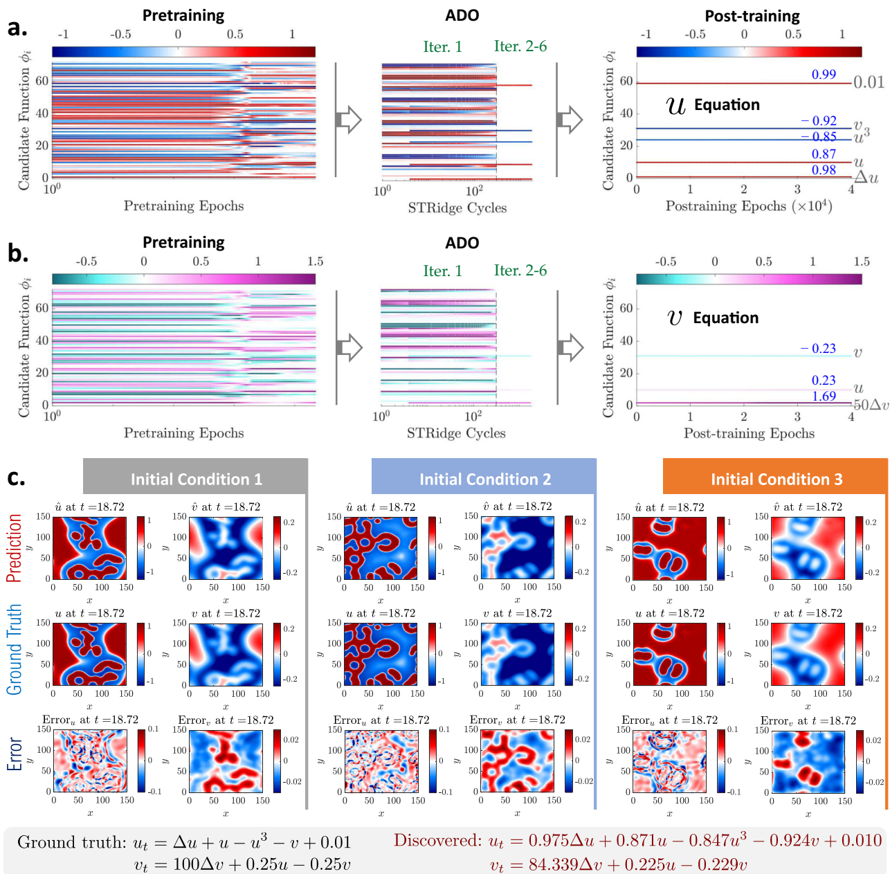
Fig. 4 Discovered Fitzhugh-Nagumo equations based on data sampled under three initial conditions (ICs) with 10% noise. a Evolution of the sparse coefficients \lambda_u \in \mathbb{R}^{72 \times 1} for 72 candidate functions used to construct the first PDE ( u -equation), where the color represents the coefficient value. b Evolution of the sparse coefficients \lambda_v \in \mathbb{R}^{72 \times 1} for the second PDE ( v -equation). For visualization purpose, we re-scale the identified coefficients of the constant stimulus term “1” in the u -equation by multiplying 100 and of the diffusion term \Delta v in the v -equation by dividing 50. c Snapshots of predicted response, ground truth and error distributions for all three ICs at an unmeasured time instance ( t = 18.72 ). The relative \ell_2 error for the predicted full-field response (stacked u and v ) is 5.02%.
