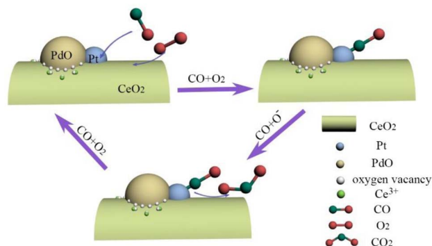
Scheme 1 A possible mechanism for catalytic CO oxidation on (\text{Pt-Pd})/\text{CeO}_2 catalyst.
