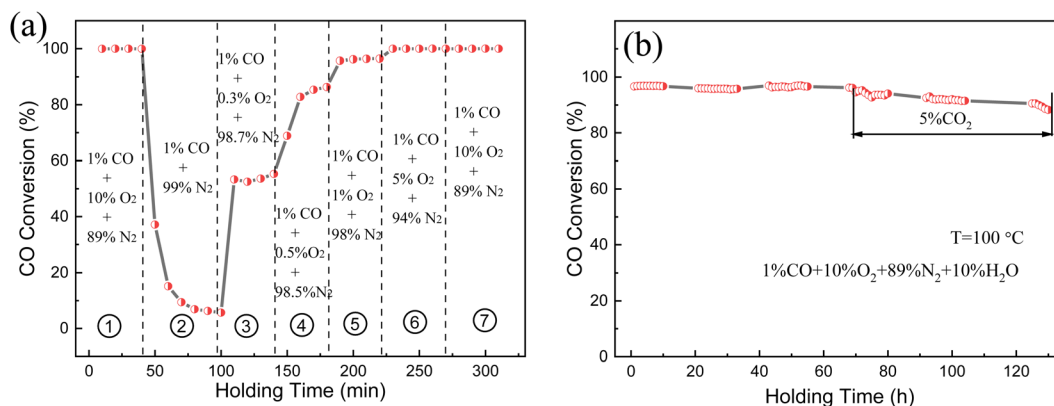
Fig. 9 (a) Catalytic performance under varied oxygen concentrations and (b) long-term stability of the (\text{Pt}_{0.1}\text{-Pd}_{0.2})/\text{CeO}_2 -573 K catalyst.
