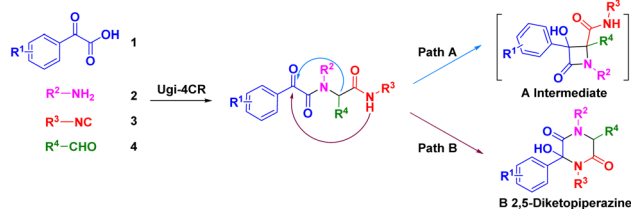
Scheme 2 Nucleophilic attack of carbanion (path A) or secondary amide (path B).
