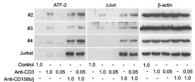
Figure 7. Stimulation of CD158j in CD4 + CD28 null T cells leads to expression of ATF-2 and c-Jun. CD4 + CD28 null CD158j + T cell clones (clones #2, #3, #4), and Jurkat T cells expressing CD158j were stimulated with anti-CD3 and/or anti-CD158b/j mAbs and cross-linked with rabbit anti-mouse IgG Ab. After SDS-PAGE and transfer to a nitrocellulose membrane, the cell lysates were analyzed for expression of ATF-2 and c-Jun. The membranes were stripped and reprobed with Ab against \beta -actin.
