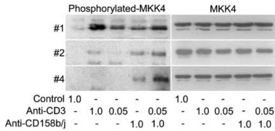
Figure 5. Stimulation of CD158b/j in CD4 + CD28 null T cells leads to MKK4 phosphorylation. CD4 + CD28 null CD158j + T cell clones (clones #1, #2, and #4) were stimulated with anti-CD3 and/or anti-CD158b/j mAbs and cross-linked with rabbit anti-mouse IgG Ab. After SDS-PAGE and transfer to a nitrocellulose membrane, the cell lysates were analyzed for phosphorylation of MKK4 (left panels). The blots were stripped and reprobed with Ab against total MKK4 (right panels).
