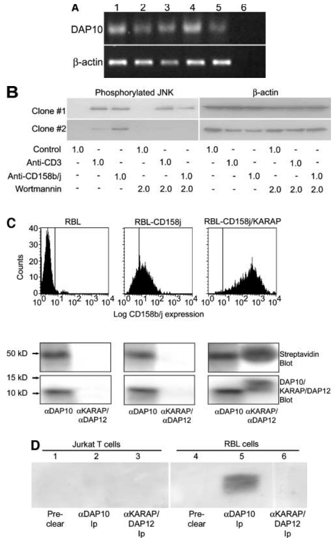
Figure 9. CD158j and DAP10 do not associate. RT-PCR was used to amplify transcripts for DAP10 from PBMCs (lane 1) and CD4 + CD28 null T cell clones (lanes 2–5). cDNA was omitted for the negative control (lane 6) (A). CD4 + CD28 null CD158b/j + T cell clones were stimulated with anti-CD3 or anti-CD158b/j in the presence or absence of 2.0 μM wortmannin. After SDS-PAGE and transfer to a nitrocellulose membrane, the cell lysates were analyzed for phosphorylation of JNK (left panels). The blots were then stripped and reprobbed with Abs against β-actin (right panels). Results from two T cell clones are shown (B). DAP10-expressing RBL cells (left panel) were stably transfected with CD158j alone (middle panel) or with CD158j and KARAP/DAP12 (right panel). Cell surface expression of CD158j was confirmed by flow cytometry (top panels). DAP10 or KARAP/DAP12 was immunoprecipitated from lysates of biotinylated transfected RBL cells. After SDS-PAGE and transfer to nitrocellulose membranes, coimmunoprecipitated cell-surface proteins were detected by streptavidin-HRP (middle panels). Immunoprecipitation of DAP10 and KARAP/DAP12 was confirmed by immunoblot with anti-DAP10 or anti-KARAP/DAP12 Ab (bottom panels) (C). DAP10 or KARAP/DAP12 was immunoprecipitated from Jurkat T cells (lanes 1–3) or RBL cells (lanes 4–6). After SDS-PAGE and transfer to a nitrocellulose membrane, samples (protein-G pre-clear, lanes 1 and 4; DAP10 immunoprecipitate, lanes 2 and 5; KARAP/DAP12 immunoprecipitate, lanes 3 and 6) were analyzed by Western blot using DAP10 Ab (D).
