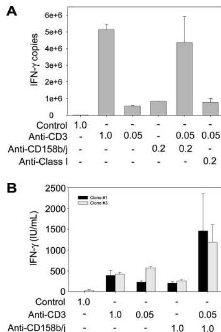
Figure 2. CD158b/j costimulates expression of IFN- \gamma in CD4 + CD28 null T cells. CD4 + CD28 null CD158b/j + T cell clones were stimulated using immobilized mouse IgG and anti-CD3 mAb alone or in combination with anti-CD158b/j mAb (shown as \mu g/ml). The number of IFN- \gamma transcripts was quantified using real-time PCR. Anti-MHC mAb is included as a negative control (A). Cells were stimulated as above and IFN- \gamma cytokine production was quantified by ELISA (B).
