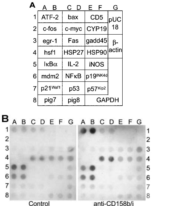
Figure 3. Stimulation through CD158b/j results in an up-regulation of ATF-2 and HSP27 transcripts. The PathwayFinder cDNA Array is spotted in duplicate with 23 cDNAs. Represented on the membrane are the ERK (egr-1 and c-fos), JNK (ATF-2, hsf1, HSP27, and HSP90), NF- \kappa B (iNos, NF- \kappa B, and I \kappa B \alpha ), NFAT (IL-2, Fas, and CD5), TGF- \beta (p16, p21, and p57 Kip2 ), Wnt (c-myc), p53 (p21, gadd45, pig7, pig8, mdm2, and bax), and CREB pathways (egr-1, CYP19, and c-fos). The membrane also included a negative control (pUC18) and two positive controls ( \beta -actin and GAPDH) (A). A CD4 + CD28 null CD158b/j + T cell clone was stimulated with control mouse IgG or anti-CD158j mAb and cross-linked with rabbit anti-mouse IgG Ab. Total RNA was harvested and used to probe the PathwayFinder cDNA Array (B).
