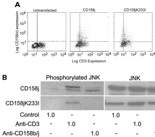
Figure 8. Mutation of transmembrane lysine residue in CD158j abolishes ability to induce JNK phosphorylation. Jurkat T cells were transiently transfected with constructs containing the CD158j cDNA or the CD158j233I cDNA. Cell-surface expression was confirmed by flow cytometry (A). Jurkat T cells transfected with either CD158j or CD158jK233I were stimulated with anti-CD3 or anti-CD158b/j mAb and cross-linked with rabbit anti-mouse IgG Ab. After SDS-PAGE and transfer to a nitrocellulose membrane, the cell lysates were analyzed for phosphorylation of JNK (left panels). The blots were then stripped and reprobbed with Abs against total JNK (right panels) (B).
