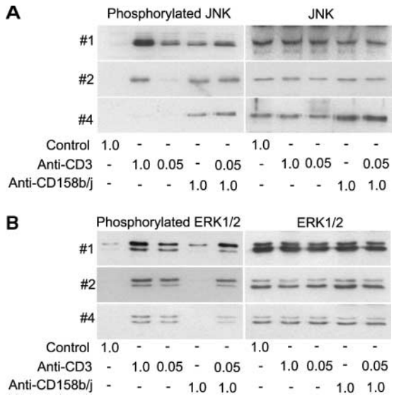
Figure 4. Stimulation of CD158b/j in CD4 + CD28 null T cells leads to JNK, but not ERK, phosphorylation. CD4 + CD28 null CD158j + T cell clones shown in Figure 1 (clones #1, #2, and #4) were stimulated with anti-CD3 and/or anti-CD158b/j mAbs and cross-linked with rabbit anti-mouse IgG Ab. After SDS-PAGE and transfer to a nitrocellulose membrane, the cell lysates were analyzed for phosphorylation of JNK (left panels), after which the blots were stripped and re-probed with Abs against total JNK (right panels) (A). After SDS-PAGE and transfer to a nitrocellulose membrane, the cell lysates were analyzed for phosphorylation of ERK (left panels), after which the blots were stripped and re-probed with Abs against total ERK (right panels) (B).
