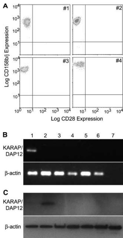
Figure 1. CD4 + CD28 null T cell clones express CD158b/j, but do not express KARAP/DAP12. CD4 + CD28 null T cells were sorted from patients with RA, and clones were established by limiting dilution. Clones were analyzed by flow cytometry for expression of CD28 and CD158b/j. Four representative clones (#1 through #4) are shown. All clones expressed CD4 (unpublished data; A). RT-PCR was used to amplify transcripts for KARAP/DAP12 and \beta -actin from PBMCs (lane 1), Jurkat T cells (lane 2), and CD4 + CD28 null T cell clones #1–#4 (lanes 3–6, respectively). cDNA was omitted for the negative control (lane 7) (B). Western blotting was used to detect KARAP/DAP12 and \beta -actin protein (bottom panels) in Jurkat T cells (lane 1), Jurkat T cells transfected with KARAP/DAP12 + vaccinia virus (lane 2), and CD4 + CD28 null T cell clones (lanes 3–7) (C).
