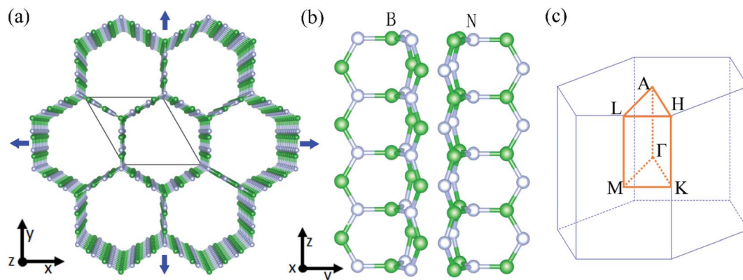
Fig. 1 (a) Perspective view of boron nitride honeycomb (BNHC) structure with its B and N linkages shown in detail in (b). The B and N atoms are represented by green and gray spheres, respectively. The blue arrows mean that the strain are loaded isotropically in all directions. (c) The first Brillouin zone with high symmetry points and routines noted.
