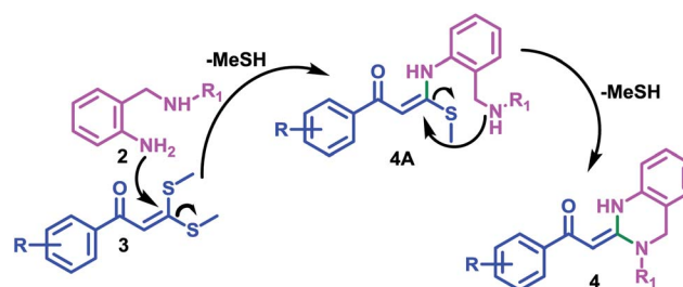
Scheme 2 Plausible Mechanism.
