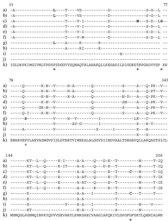
Figure 2 Amino acid sequences of DHPS from Neisseria Alignment of deduced amino acid sequences from internal fragments of folP -genes from Neisseria : a) isolate 10B:1 (Su R clone I); b) isolate 102A:2 (Su R clone III); c) isolate 102A:1 (Su R clone II); d) isolate 102A:3 (Su S ); e) isolate 10C:1 (Su S ); f) isolate 102B:3 (Su S ); g) N. meningitidis 3976 (Su R )[1]; h) N. meningitidis BT054 (Su S )[5]; i) N. mucosa ; j) N. subflava ; k) N. sicca . Amino acid residues discussed in the text are bolded and marked with * below the sequences. Accession numbers in the EMBL database are AJ457071, AJ457074, AJ457073, AJ457075, AJ457072, AJ457076, X87405, X68067, AJ457077, AJ457079 and AJ457078, respectively.
