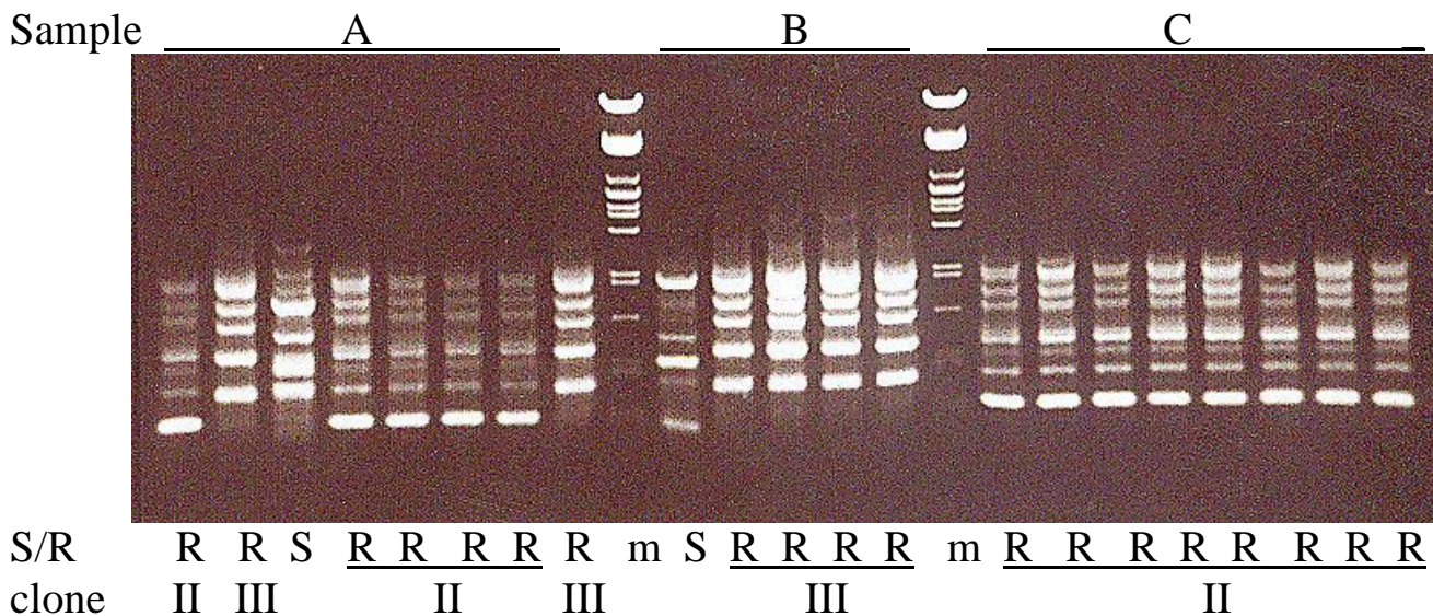
Figure 1 AP-PCR patterns of Neisseria isolates The isolates were obtained from samples collected from the same patients at three separate occasions: sample A at time zero, sample B two weeks later and sample C one year later. Sulphonamide sensitive isolates are marked with S. Resistant isolates are marked with R and the clone to which they belong. m=molecular size markers
