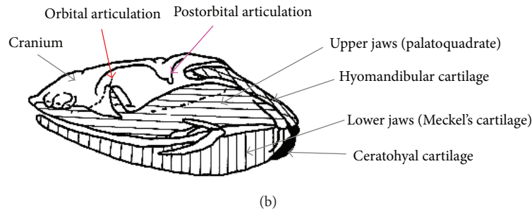
FIGURE 3: Morphological character evolution mapped onto the phylogenetic tree derived in this study (a) and structure of jaw suspension of C. anguineus (b). (a) Divergence time for each node of Selachii was estimated by the divergence time of Selachii and Batoidea (213.4 Mya (203.3~228.8 Mya in the 95% confidence intervals)) [24]. The red line extending from the circled node indicates the evolutionary time (115.4 Mya) of the divergence of Hexanchiformes from the other Squalomorphi lineages. Numbers above the branches indicate the gill cleft numbers, and numbers above the nodes indicate range of the divergence time. The schematic diagrams of jaw suspension were based on previous reports [3, 13, 25]. (b) Vertical, horizontal, and grid-lined areas and black and white areas indicate lower jaws (Meckel's cartilage), upper jaws (palatoquadrate), hyomandibular and ceratohyal cartilages, and cranium, respectively. Red and orange arrows in the schematic diagram of the jaw suspension apparatus indicate orbital and postorbital articulations, respectively.
