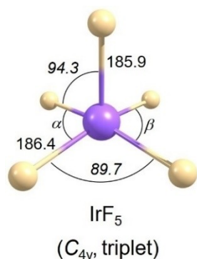
Figure 3. Computed structure of molecular IrF 5 at the 2c-X2C-B3LYP/x2c-TZVPall-2c level. Selected bond lengths (pm) and angles ( ^\circ , in italics ) are shown. The computed structures of other iridium fluorides at this level are shown in Figure S3.
