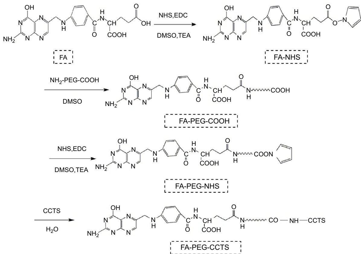
Figure S1 Synthesis of FA-PEG-CCTS conjugates.
