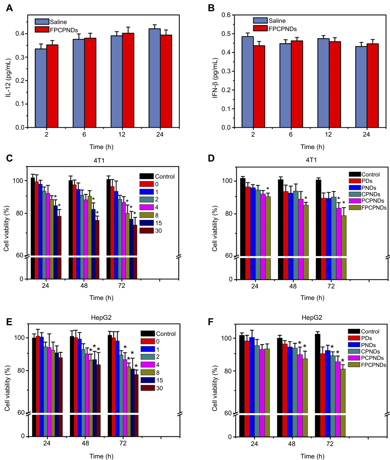
Figure 4 Evaluation of immunogenicity in vivo and cytotoxicity in vitro. The content change of (A) IL-12 and (B) IFN- \beta in mice after injected with FPCPNs (N/P=15). In vitro cytotoxicity study of (C, E) FPCPNs at different N/P ratios, and (D, F) different formulations at an N/P ratio of 15 against HepG2 and 4T1 cells by MTT assay. * P <0.05.
