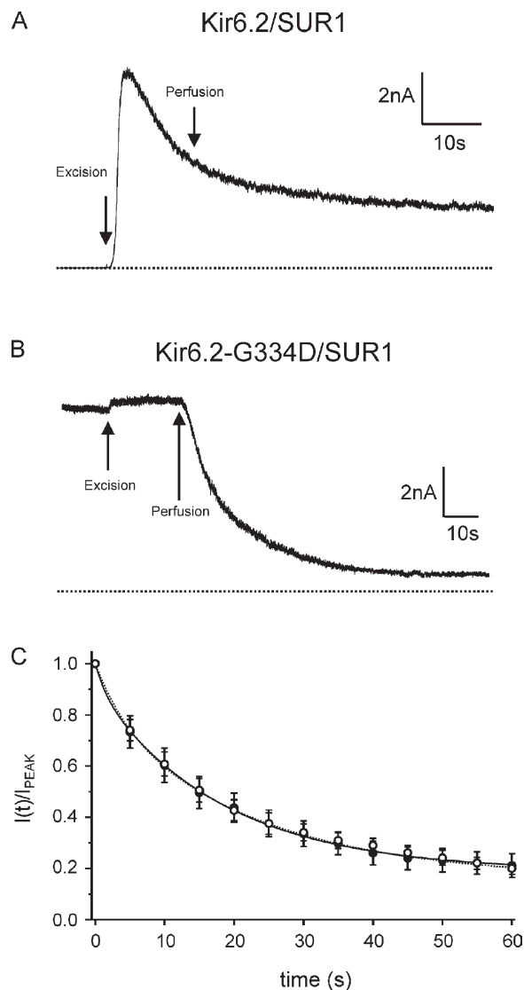
Figure 2. Rundown of Kir6.2/SUR1 and Kir6.2-G334D/SUR1 channels in macropatches. (A) Macroscopic Kir6.2/SUR1 currents at -60 mV recorded from a giant patch. Patch excision and the start of the perfusion with nucleotide-free intracellular solution are indicated by the arrows. The dotted line represents the zero current level. (B) Macroscopic Kir6.2-G334D/SUR1 currents recorded at -60 mV. Patch excision and the start of the perfusion with nucleotide-free solution are indicated by the arrows. The dotted line represents the zero current level. (C) Mean macroscopic K_{ATP} current at -60 mV during the first 60 s of rundown, expressed as a fraction of the maximum value reached after excision, is plotted as a function of the time after patch excision for Kir6.2/SUR1 (open circles; n = 10 ) and Kir6.2-G334D/SUR1 channels (filled circles; n = 10 ). The lines are the best fit of a double-exponential function to the mean data (solid line, Kir6.2/SUR1; dotted line, Kir6.2-G334D/SUR1).
