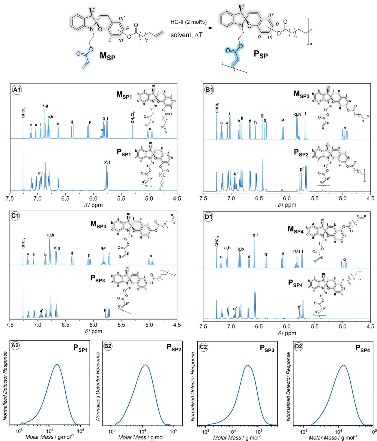
Fig. 2 Synthesis and characterization of main-chain spiroopyran-based polymers. Top: synthesis via head-to-tail ADMET polymerization and ^1\text{H} NMR sectional spectra (600 MHz, 32 scans, \text{CDCl}_3 ) of monomers and polymers: (A1) \text{M}_{\text{SP1}} and \text{P}_{\text{SP1}} , (B1) \text{M}_{\text{SP2}} and \text{P}_{\text{SP2}} , (C1) \text{M}_{\text{SP3}} and \text{P}_{\text{SP3}} , (D1) \text{M}_{\text{SP4}} and \text{P}_{\text{SP4}} . Full 1D and 2D NMR spectra are provided in the ESI, Section 9.† The assignment of the proton resonances was assisted through the analysis of 1D and 2D NMR spectra of precursors and desired products as described in ESI, Section 9.† Details of the polymerization conditions can be found in the ESI, Section 2.† Bottom: dimethylacetamide (DMAc)-size exclusion chromatography (SEC) traces of \text{P}_{\text{SP1}} (A2), \text{P}_{\text{SP2}} (B2), \text{P}_{\text{SP3}} (C2) and \text{P}_{\text{SP4}} (D2).
