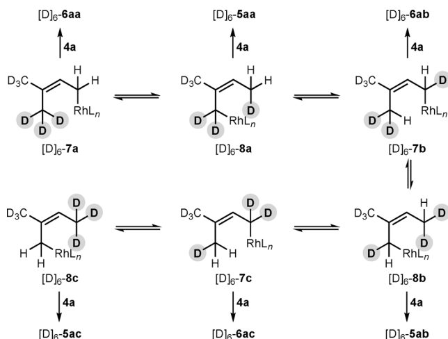
Scheme 7. Deuterium–hydrogen exchange through the reversible 1,4- \text{Rh}^{\text{I}} migration of allylrhodium species [D]_6\text{-7} and [D]_6\text{-8} .
