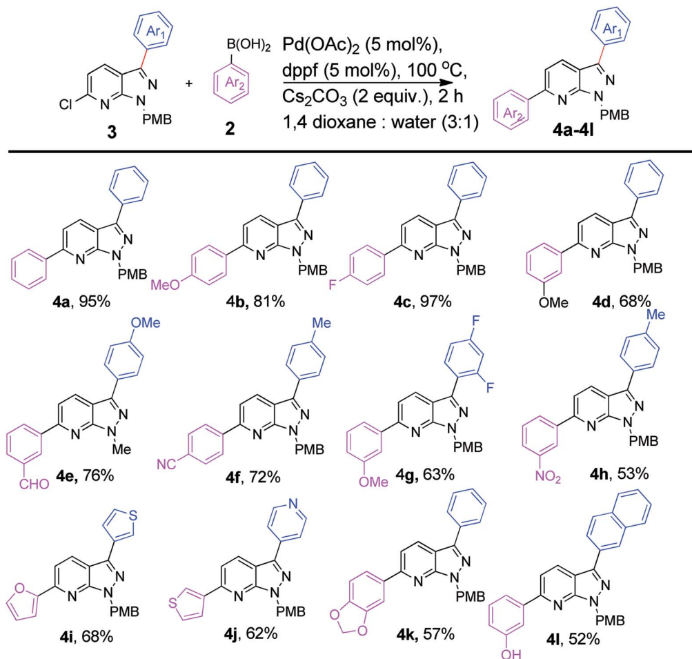
Scheme 2 Pd-catalyzed C6-arylation of 3-arylpyrazolo[3,4- b ]pyridines. a,b Reaction conditions: 6-chloro-1-(4-methoxybenzyl)-3-phenyl-1 H -pyrazolo[3,4- b ]pyridine 3 (1.0 equiv.), arylboronic acid 2 (1.0 equiv.), Pd(OAc) 2 (5 mol%), dppf (5 mol%), Cs 2 CO 3 (2.0 equiv.), 1,4-dioxane : water (3 : 1) (5 mL), 100 °C, 2 h; b isolated yields.
