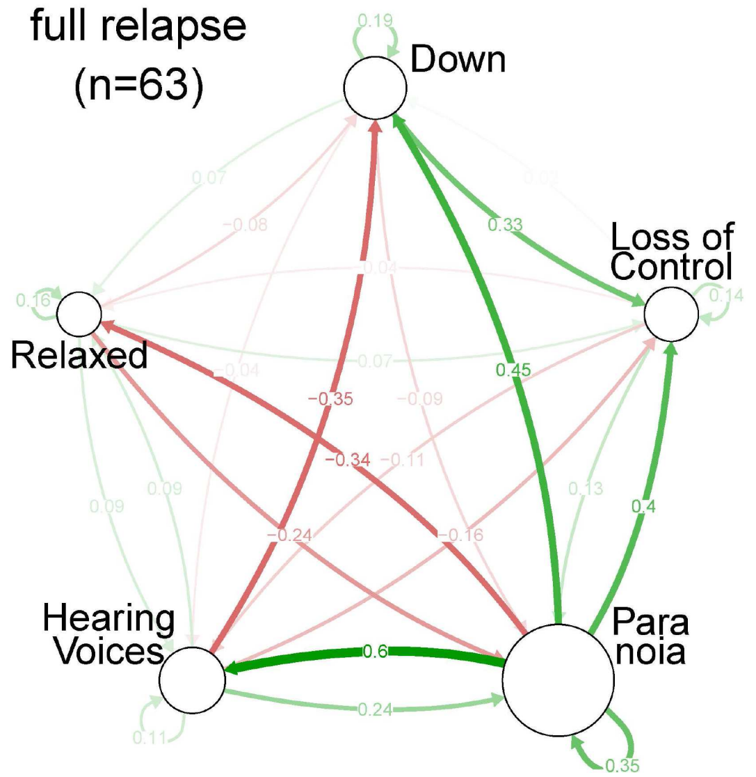
Fig 4. Centrality indices per symptom, for each of the three strata of severity: relapse state.
