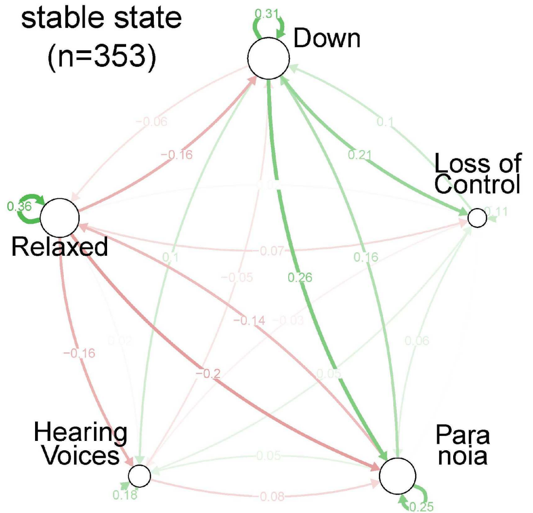
Fig 2. Centrality indices per symptom, for each of the three strata of severity: stable state.
