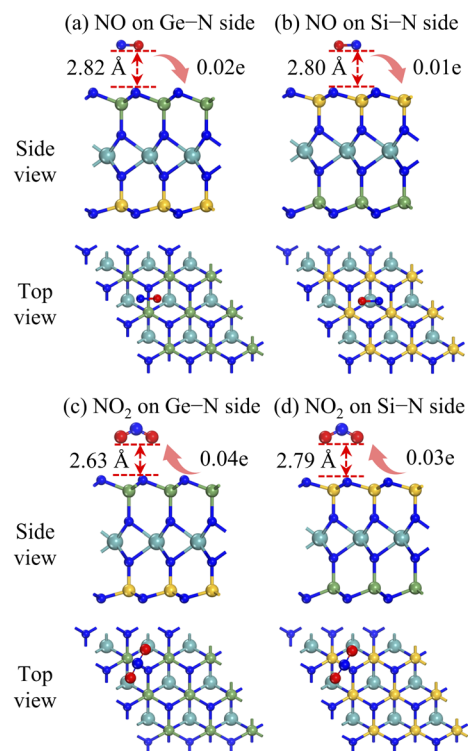
Fig. 4 Side and top views of the most stable adsorption configurations of the Janus MoSiGeN 4 monolayer adsorbed (a, b) NO or (c, d) NO 2 molecules. Here, the orientation and values of charge transfer are also denoted.
