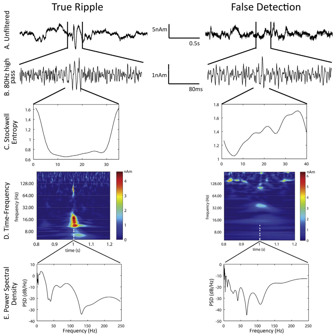
Fig. 2. Schematic overview of automatic ripple detection algorithm, with examples of a true ripple (left) and an event that is not in the final output of the detector (right), because the entropy is not stable over the length of the event. A) Unfiltered virtual sensor signal. B) 80 Hz high-pass filtered signal, showing the true ripple (left) and false detection (right). C) Stockwell entropy over the length of the event is stable for the true ripple (left), and irregular for the false detection (right). D) Time-frequency decomposition shows a high frequency component for the true ripple (~100 Hz) and the spike that can be seen in part A (12–20 Hz, left), and less distinct components and high frequency artefacts for the false detection (right). E) The power spectral density (PSD) also shows the high frequency component in the true ripple (60–100 Hz, left), and the irregular high frequency activity for the false detection (right).
