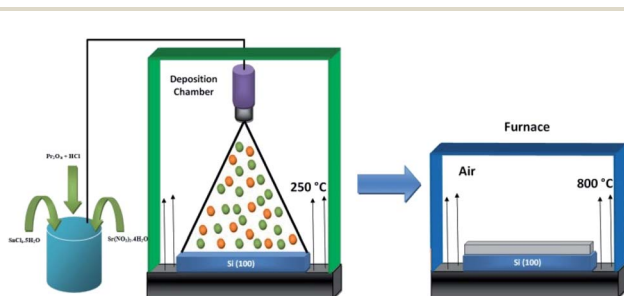
Fig. 1 Schematic illustration of the deposition set-up with the different steps followed.
