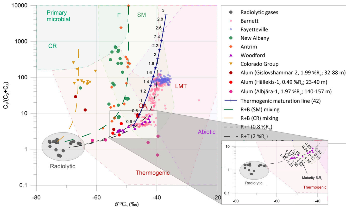
Fig. 1. Revised Bernard plot after Milkov and Etiope (5). Dark blue line indicates a thermogenic maturation line according to ref. 6 with % R_0 increasing from 0.6 to 3. Black dashed lines indicate mixing of radiolytic (R) and thermogenic (T) gas components; the green dashed line indicates the mixing of radiolytic gas with a mixture of primary biogenic gas (e.g., methyl type fermentation) and/or secondary microbial gas (both marked as B in the legend). The brown dashed line indicates mixing of radiogenic (R) and microbial gas derived by \text{CO}_2 reduction. CR, \text{CO}_2 reduction; F, methyl-type fermentation; SM, secondary microbial; OA, oil-associated (midmature) thermogenic gas; LMT, late mature thermogenic gas after Milkov et al. (1). (Inset) Data points from the Woodford Shale with maturities (7) increasing toward lower dryness values. Data are from radiolytic gases (8) and Barnett and Fayetteville (9), Antrim (10), New Albany (11), Woodford (7), Colorado Group (12), and Alum (13) shales.
