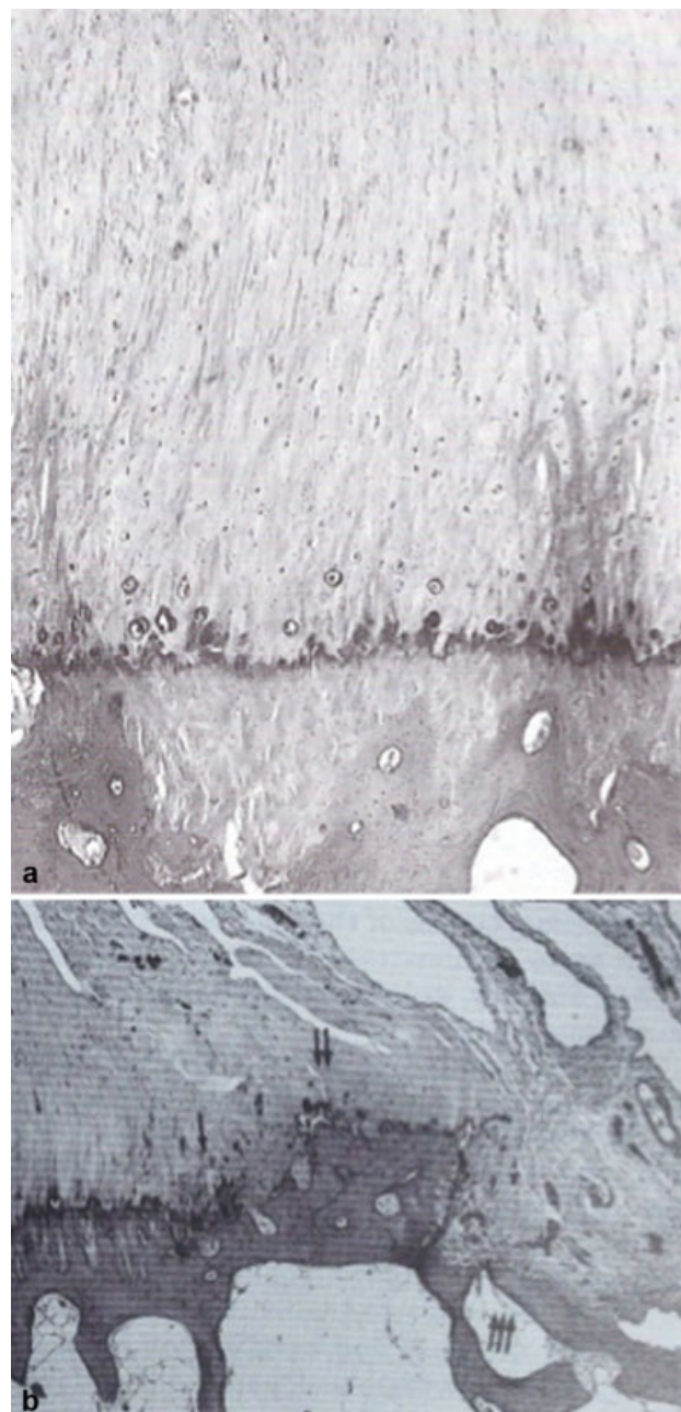
Fig. 2 Organization of the fibers of the supraspinatus tendon in layers in the young, and its progressive disorganization in the adult.
