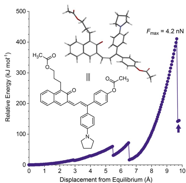
Fig. 1 Density functional theory (DFT) calculations using the constrained geometries simulate external force (CoGEF) method performed on a linear 2 H -naphtho[2,3- b ]pyran model containing a para -pyrrolidine substituent predict a ring-opening reaction upon mechanical elongation. The structure of the predicted merocyanine product is shown, corresponding to the position in the profile denoted by the arrow. The features at ~5.5 and 6.5 Å displacement correspond to conformational changes. Calculations were performed at the B3LYP/6-31G* level of theory.
