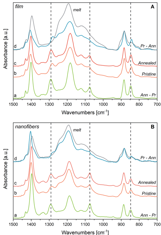
Fig. 4 Panel A: P(VDF-TrFE) film, (a) spectrum obtained as the difference between the IR spectrum after annealing (annealed, c) and that of the same sample before annealing (pristine, b); (d) difference between the IR spectrum before annealing (pristine, b) and that of the sample after annealing (annealed, c). On spectrum (d) is also reported in grey the spectrum of the melt. Panel B: same difference spectra (a), (d) for P(VDF-TrFE) nanofibers. Spectra of the samples at room temperature, pristine (b) and annealed (c) and of the melt (d, grey) are reported for sake of comparison. Spectra normalized on 883\text{ cm}^{-1} peaks.
