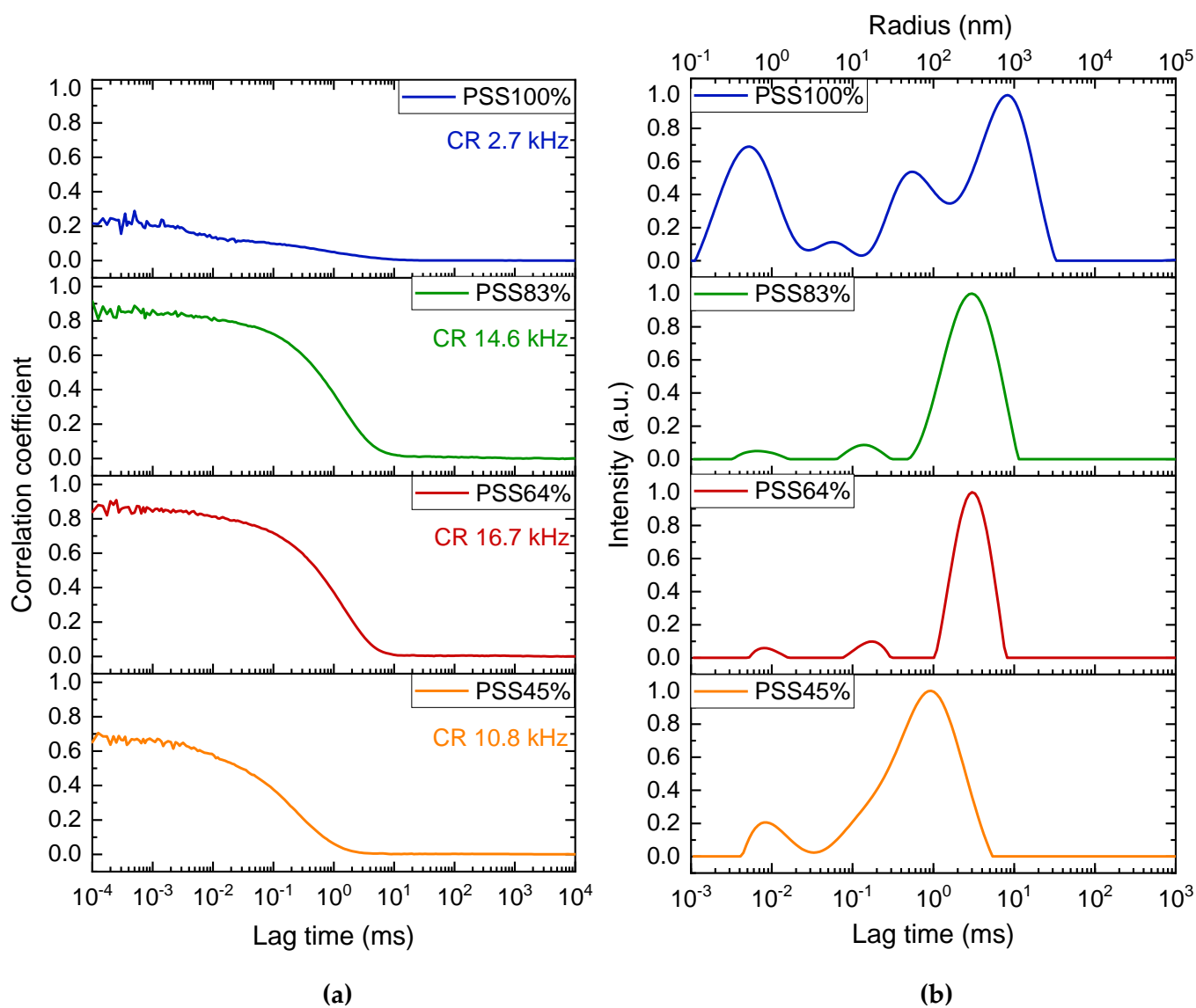
Figure 3. DLS analysis of aqueous solutions of P(St-co-SSNa) varying in the degree of sulfonation. (a) Normalized intensity autocorrelation functions. The scattering intensity of P(St-co-SSNa) solutions is given as the count rate (CR) determined at 90^\circ detection angle and normalized by the polymer mass concentration (g/L). (b) Intensity-average relaxation time distributions. The corresponding unweighted radii are shown on the top axis. All PE solutions were prepared at a concentration of 6 mM in charged units.
