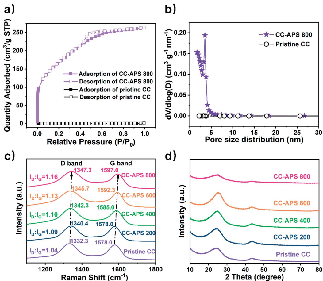
Fig. 3 (a) \text{N}_2 adsorption–desorption isotherms and (b) corresponding pore size distributions of the pristine CC and CC-APS 800, respectively. (c) Raman and (d) XRD spectra of the pristine CC, CC-APS 200, CC-APS 400, CC-APS 600, and CC-APS 800.
