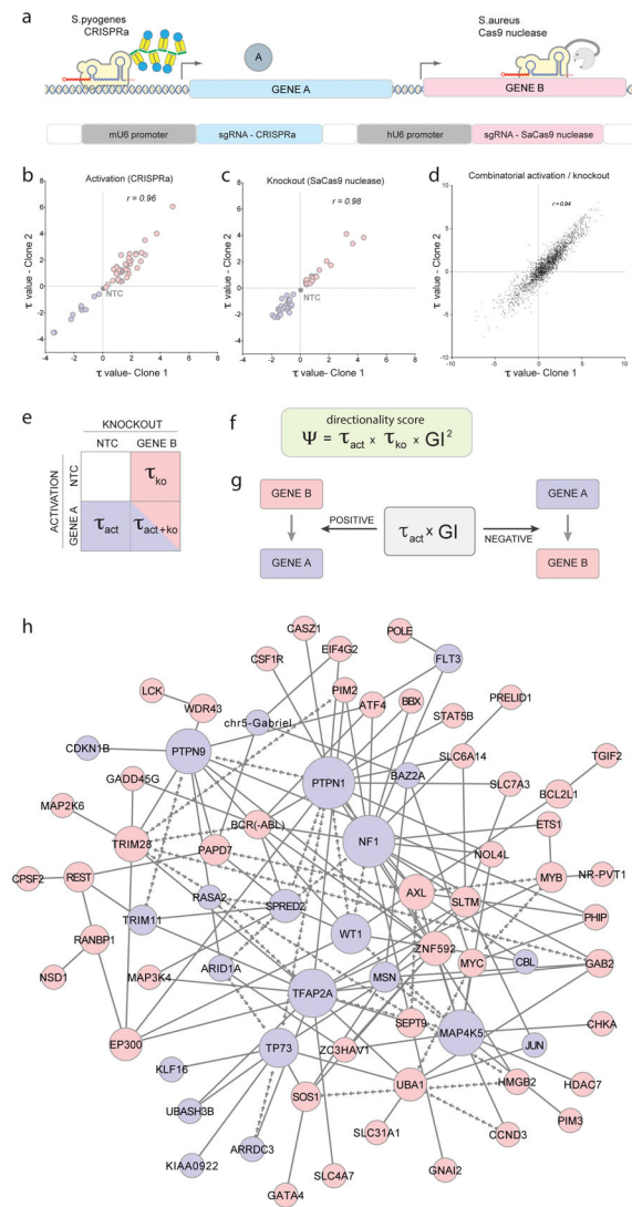
Figure 3. Orthogonal CRISPR screens can quantify directional genetic interactions a , Concept of the application of the orthogonal system for directional gene interaction studies. In the same cell, one gene is activated (CRISPRa) while another gene is knocked out (SaCas9 nuclease). b–d , Correlation of \tau values from two clonal cell line replicates is shown for b , gene activation, c , gene knockout and d , all possible combinations thereof. Correlation values ( r ) are Pearson product-moment correlation coefficients. e , Schematic of perturbation data set from each gene pair (blue = depleted, red = enriched, NTC = non-target control sgRNA) f , Formula for calculating \Psi scores. Negative \Psi scores define interactions in which directionality could be inferred. g , To determine which of both interaction partners acts up- or downstream, \tau_{\text{activation}} values were multiplied with genetic interaction scores. Positive values indicate a downstream function, negative values an upstream function of the activated gene. h , Based on GI and \Psi scores determined by the full orthogonal interaction screen, a genetic interaction model was constructed. For positive regulators of cell fitness, nodes are shown in red and negative regulators in blue. Arrow-shaped edges indicate inferred directional interactions between nodes. Line-shaped edges symbolise genetic
