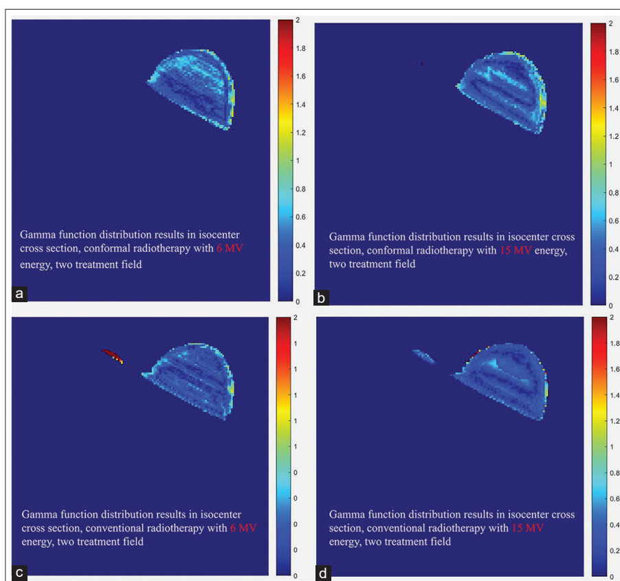
Figure 3: Gamma function distribution results in the cross-section of isocenter in the treatment planes with two treatment fields: (a) Conformal technique with 6 MV, (b) Conformal technique with 15 MV, (c) Conventional technique with 6 MV, (d) Conventional technique with 15 MV
