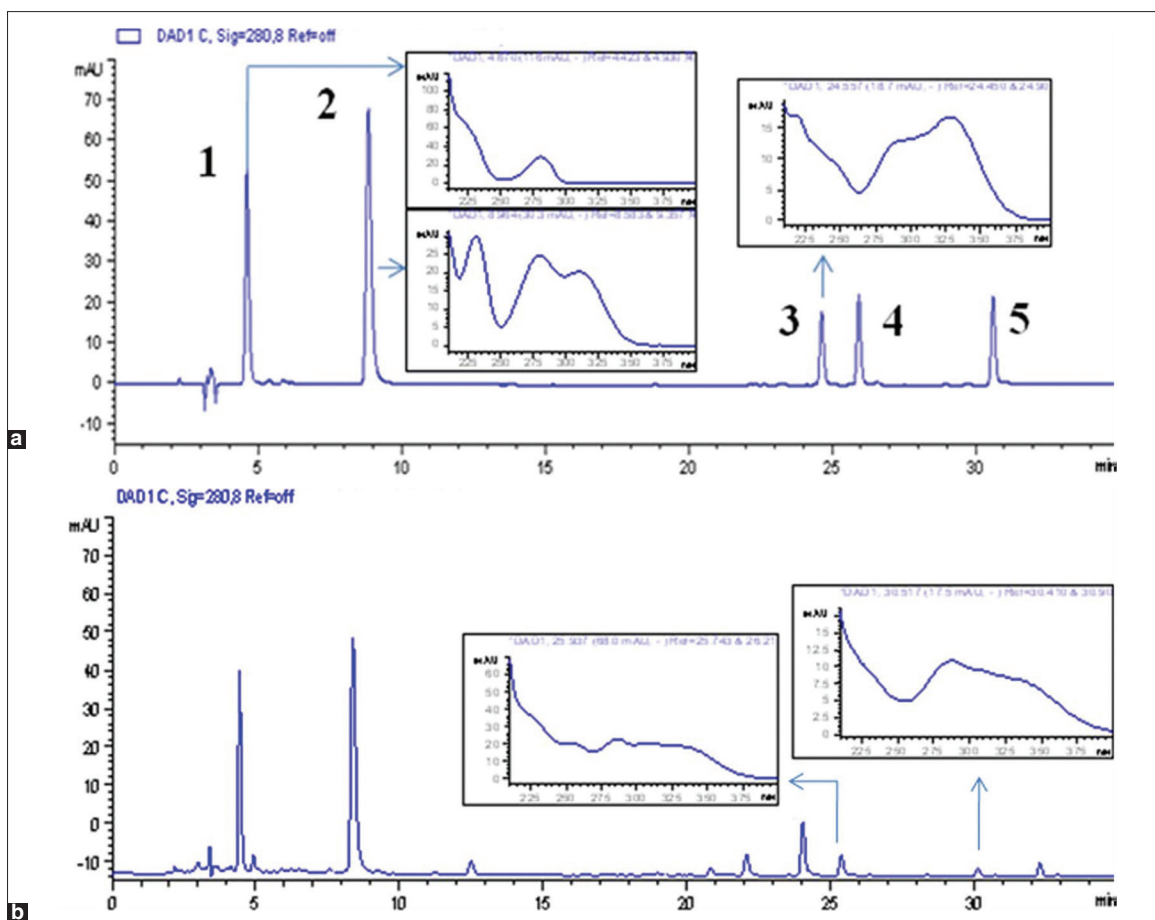
Figure 1: High-performance liquid chromatography chromatogram (280 nm) and ultraviolet spectrum of mixed standards (a) and compound Danshen injection (b). (1) Propanoid acid, (2) protocatechuic aldehyde, (3) rosmarinic acid, (4) salvianolic acid B and (5) salvianolic acid A
