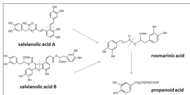
Figure 3: The degradation processes of salvianolic acid A and salvianolic acid B
