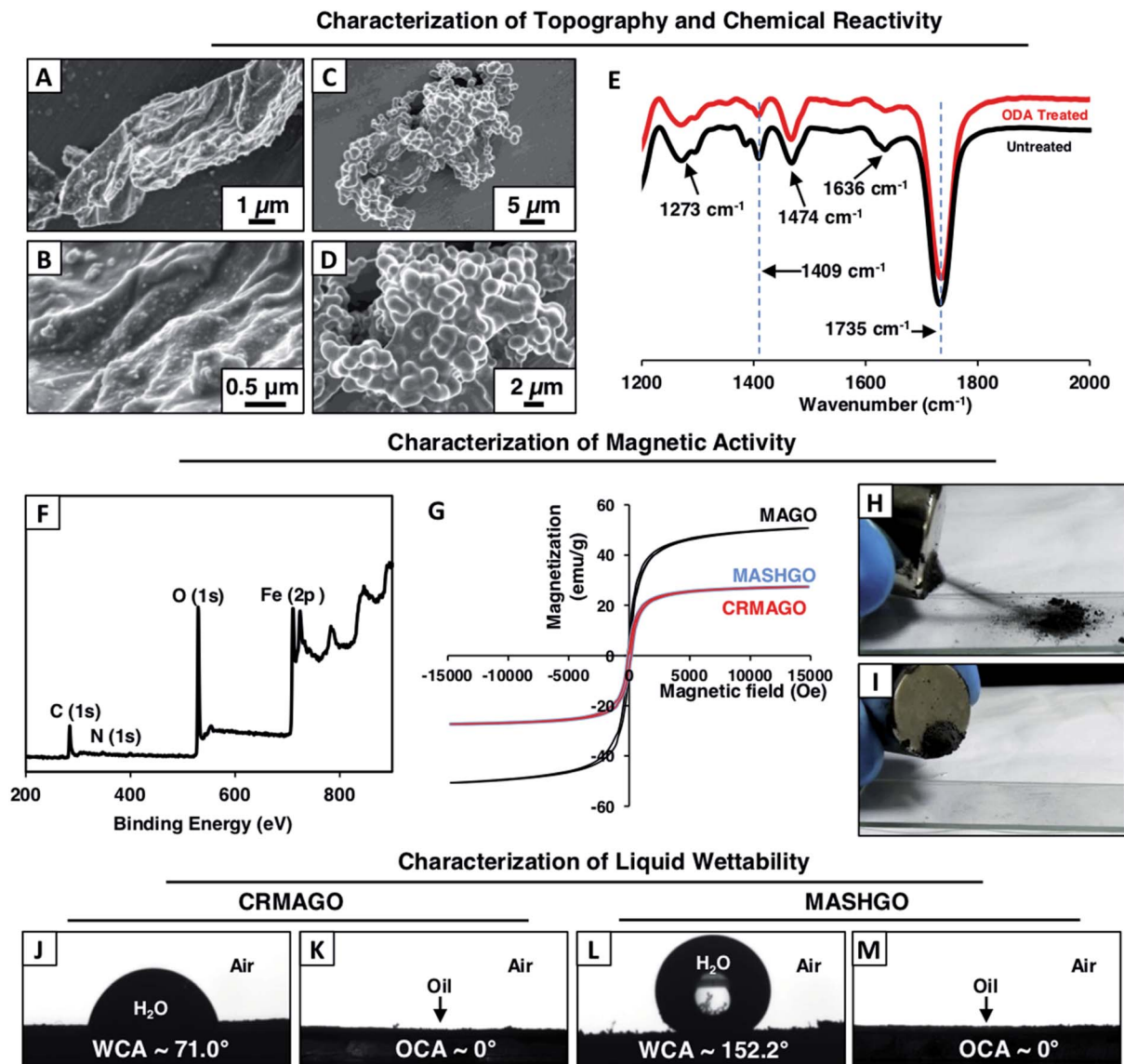
Fig. 1 (A–D) FESEM images of magnetically active graphene oxide (MAGO; (A and B)) and magnetically active superhydrophobic graphene oxide (MASHGO; (C and D)) in low (A and C) and high magnifications (B and D). (E) FTIR spectra of the chemically reactive and magnetically active graphene oxide (CRMAGO) before (black) and after (red) ODA treatment. In the FTIR spectra, the IR peak at 1735\text{ cm}^{-1} corresponds to C=O stretching. IR peaks at 1636\text{ cm}^{-1} , 1474\text{ cm}^{-1} , 1409\text{ cm}^{-1} and 1273\text{ cm}^{-1} are characteristic IR signatures for C=C stretching, C–H bending of the methylene group, C–H deformation of the \beta -carbon of the vinyl group and the C–O stretching of the ester group, respectively. (F) XPS spectra of MAGO. (G) Magnetization curves of MAGO (black), CRMAGO (red) and MASHGO (blue) at room temperature. (H and I) Digital images illustrating the collection of MASHGO using a neodymium magnet (0.5 T). (J–M) Static contact angle images of beaded water (J and L) and oil (K and M) droplets on CRMAGO (J and K) and MASHGO (L and M).
