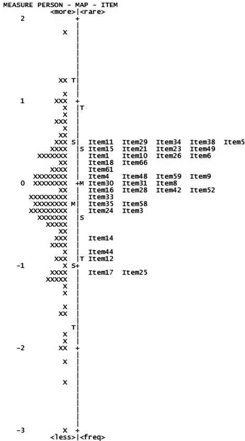
Figure. Person-ITEM map for the VILL questionnaire with 37 items.
